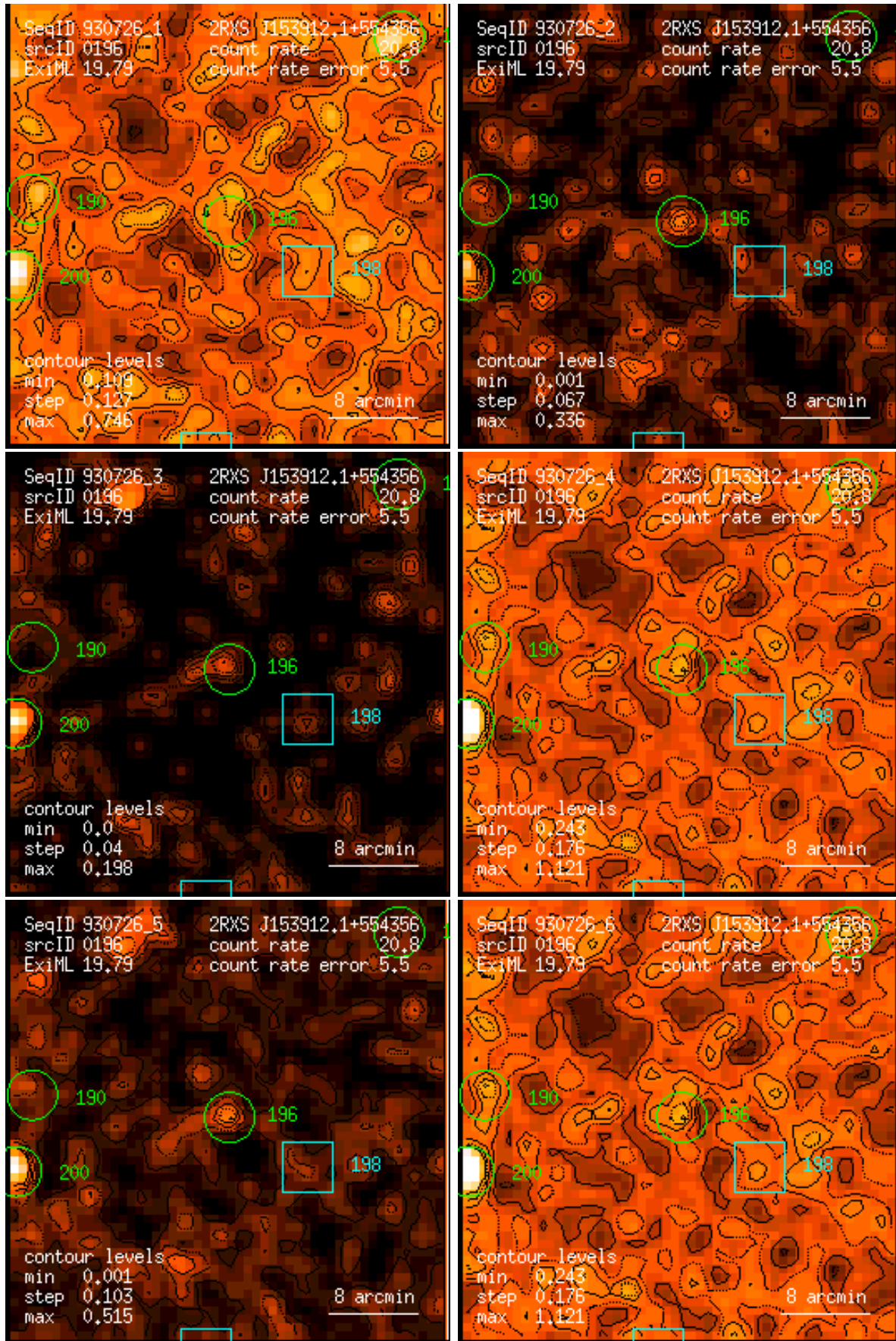
Figure 196: RASS 930726: detection 0196: band rate images, Gaussian filter: (1) PSPC channels 11 – 41, (2) 52 – 90, (3) 91 – 201, (4) 11 – 235, (5) 52 – 201, (6) 11 – 201. Broad band rates in counts/ks. Band rate contour levels in counts/ks/arcmin 2 .
