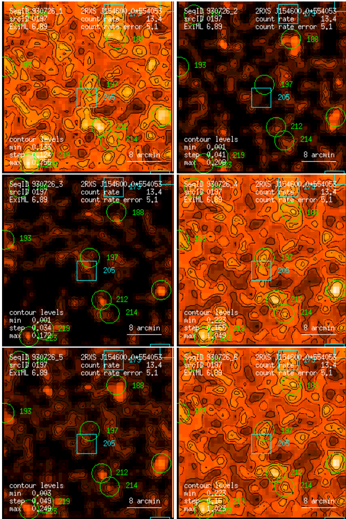
Figure 197: RASS 930726: detection 0197: band rate images, Gaussian filter: (1) PSPC channels 11 – 41, (2) 52 – 90, (3) 91 – 201, (4) 11 – 235, (5) 52 – 201, (6) 11 – 201. Broad band rates in counts/ks. Band rate contour levels in counts/ks/arcmin 2 .
