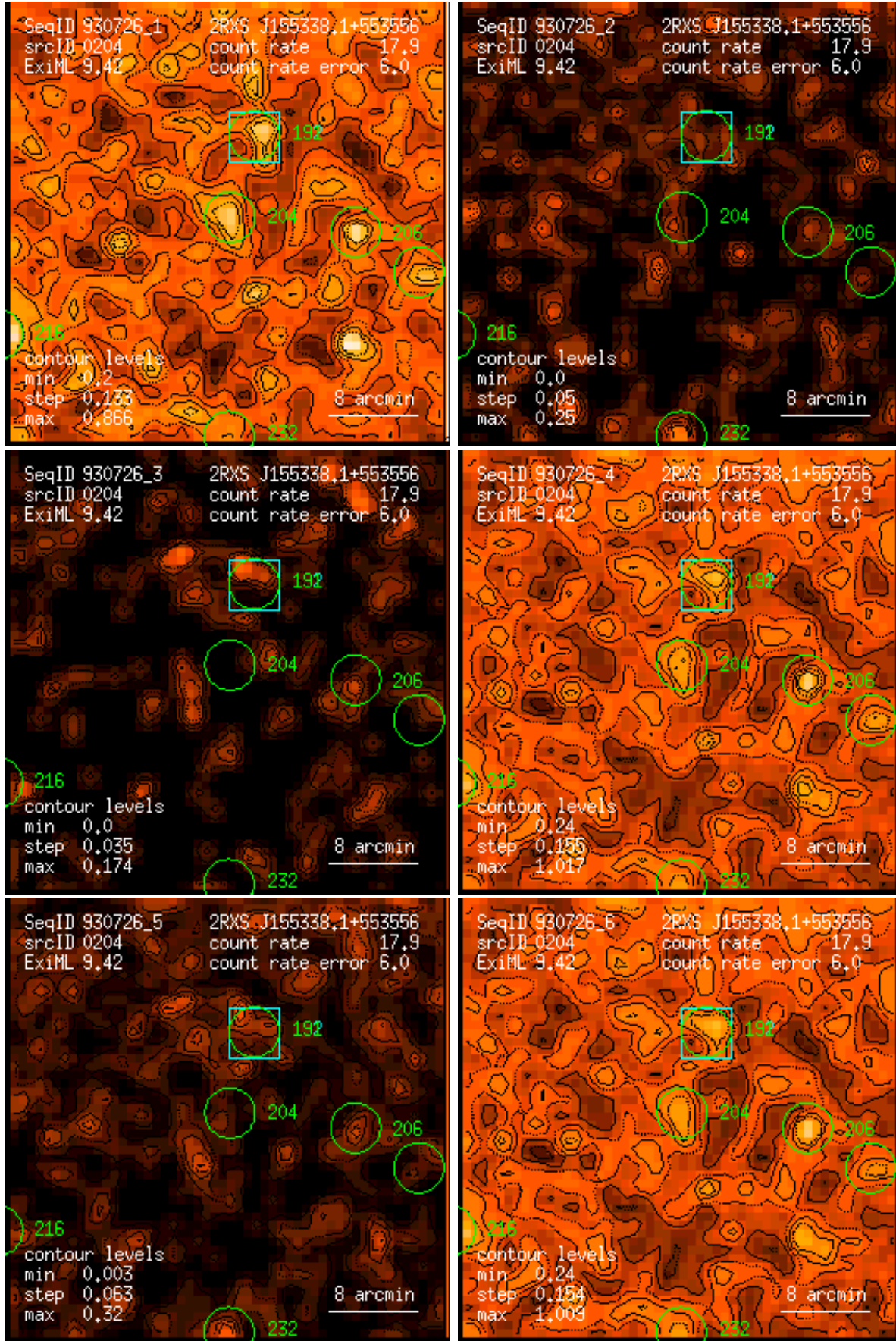
Figure 204: RASS 930726: detection 0204: band rate images, Gaussian filter: (1) PSPC channels 11 – 41, (2) 52 – 90, (3) 91 – 201, (4) 11 – 235, (5) 52 – 201, (6) 11 – 201. Broad band rates in counts/ks. Band rate contour levels in counts/ks/arcmin 2 .
