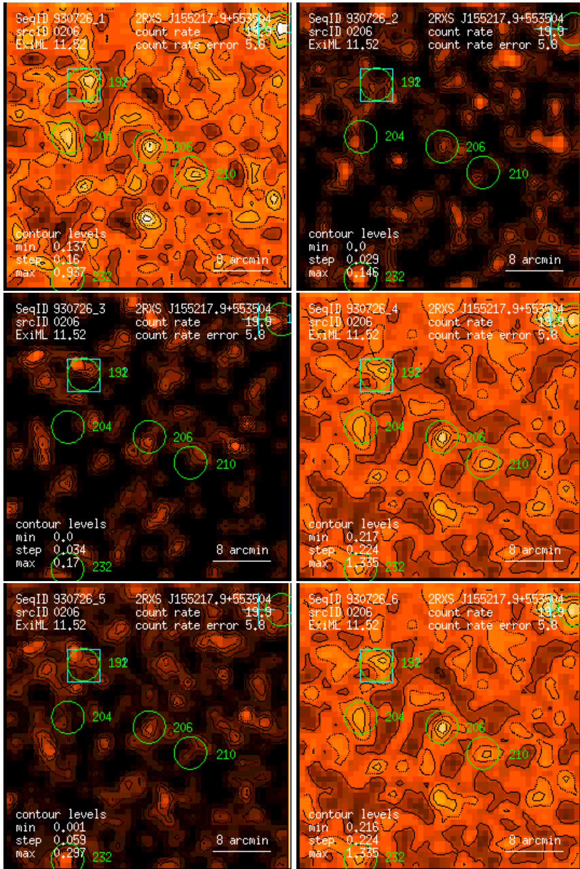
Figure 206: RASS 930726: detection 0206: band rate images, Gaussian filter: (1) PSPC channels 11 – 41, (2) 52 – 90, (3) 91 – 201, (4) 11 – 235, (5) 52 – 201, (6) 11 – 201. Broad band rates in counts/ks. Band rate contour levels in counts/ks/arcmin 2 .
