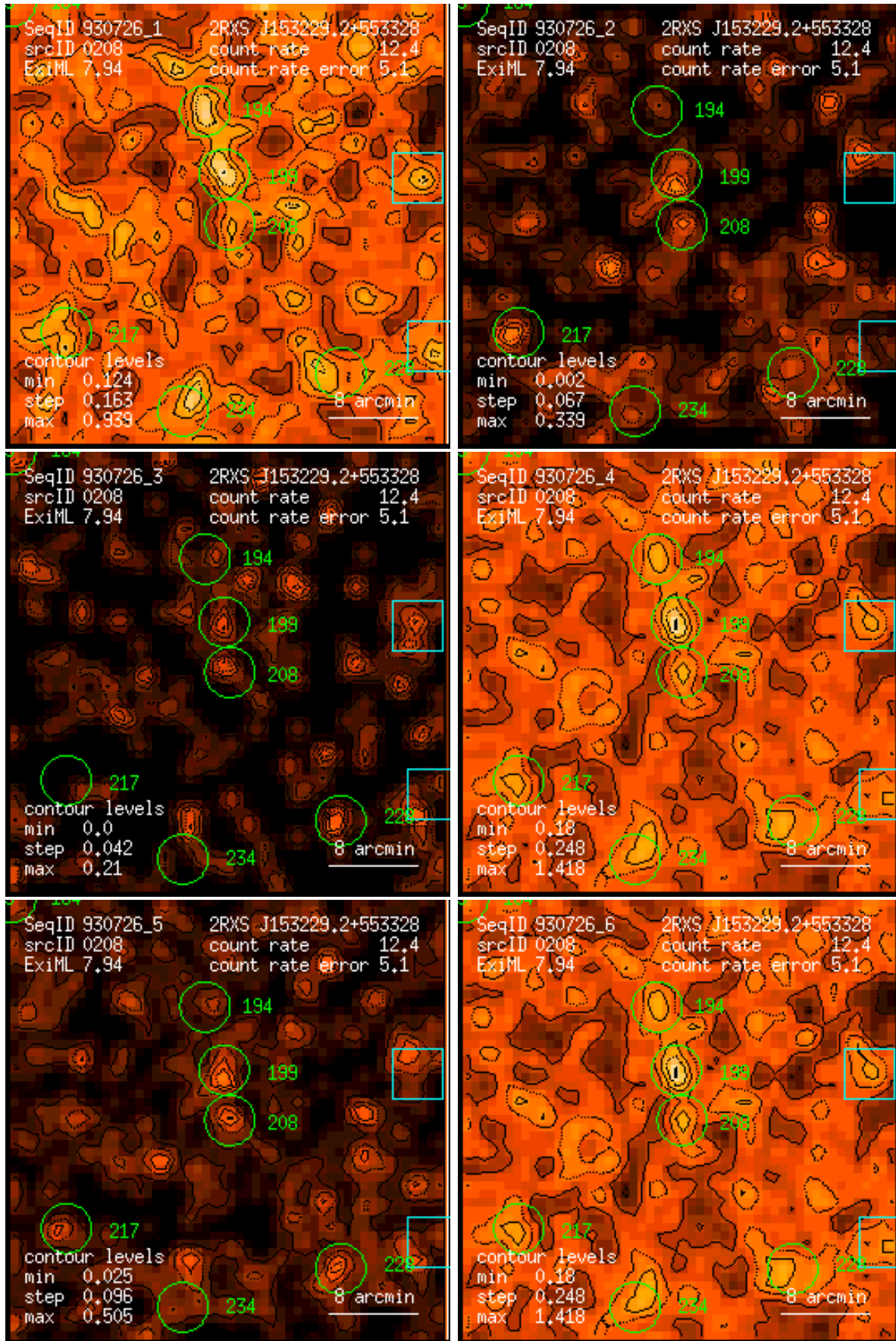
Figure 208: RASS 930726: detection 0208: band rate images, Gaussian filter: (1) PSPC channels 11 – 41, (2) 52 – 90, (3) 91 – 201, (4) 11 – 235, (5) 52 – 201, (6) 11 – 201. Broad band rates in counts/ks. Band rate contour levels in counts/ks/arcmin 2 .
