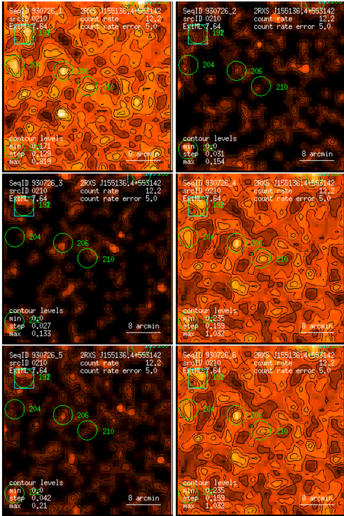
Figure 210: RASS 930726: detection 0210: band rate images, Gaussian filter: (1) PSPC channels 11 – 41, (2) 52 – 90, (3) 91 – 201, (4) 11 – 235, (5) 52 – 201, (6) 11 – 201. Broad band rates in counts/ks. Band rate contour levels in counts/ks/arcmin 2 .
