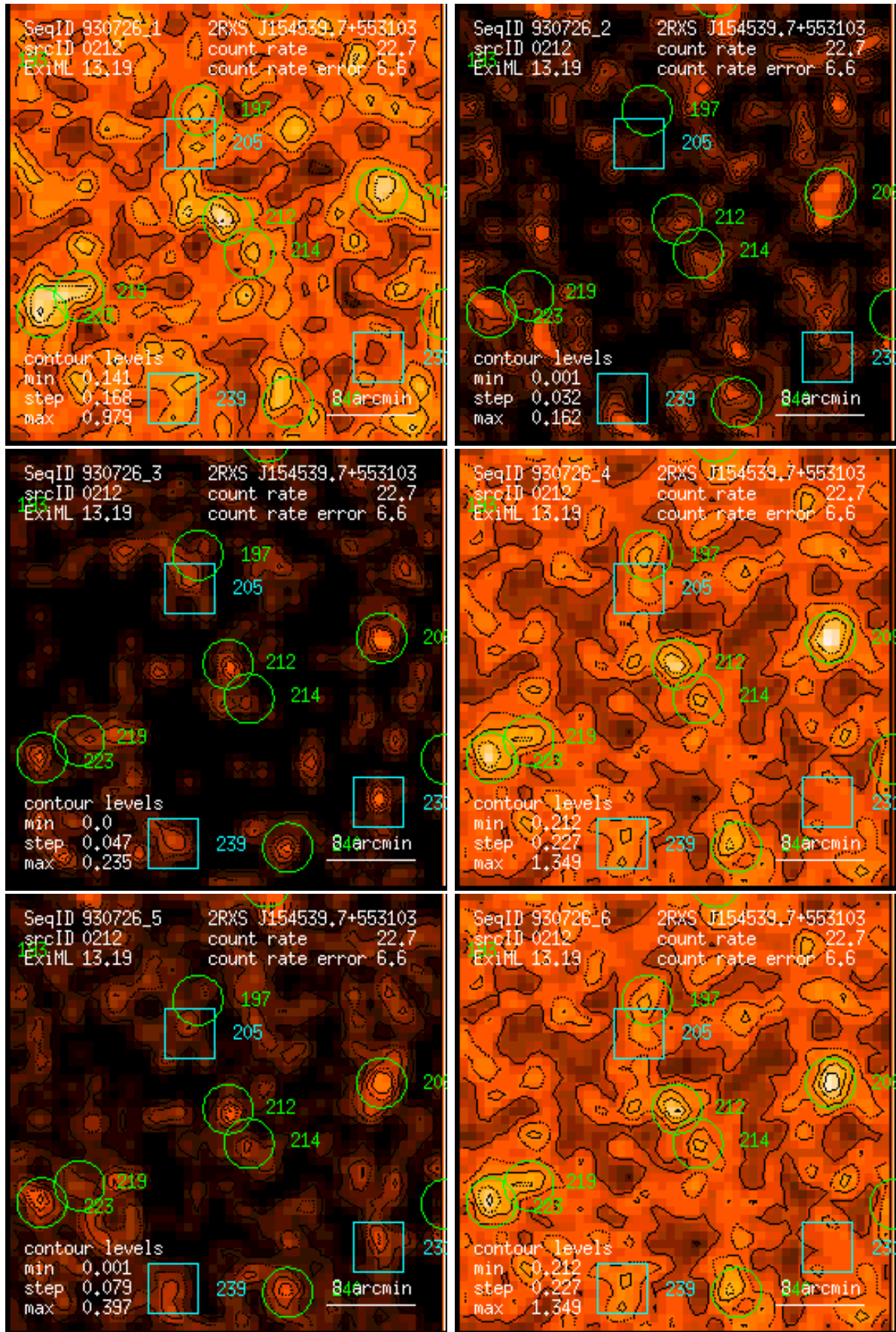
Figure 212: RASS 930726: detection 0212: band rate images, Gaussian filter: (1) PSPC channels 11 – 41, (2) 52 – 90, (3) 91 – 201, (4) 11 – 235, (5) 52 – 201, (6) 11 – 201. Broad band rates in counts/ks. Band rate contour levels in counts/ks/arcmin 2 .
