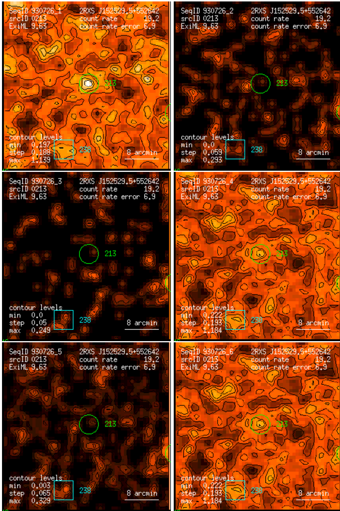
Figure 213: RASS 930726: detection 0213: band rate images, Gaussian filter: (1) PSPC channels 11 – 41, (2) 52 – 90, (3) 91 – 201, (4) 11 – 235, (5) 52 – 201, (6) 11 – 201. Broad band rates in counts/ks. Band rate contour levels in counts/ks/arcmin 2 .
