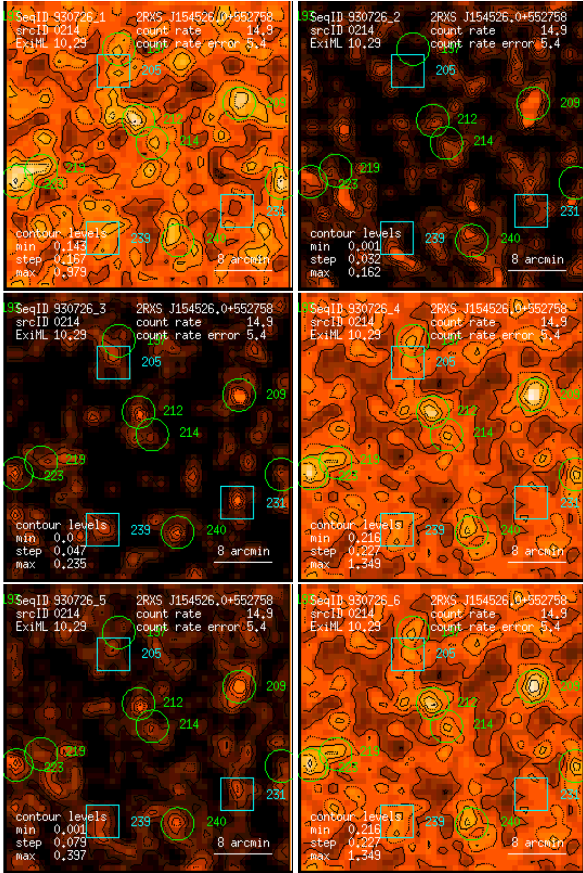
Figure 214: RASS 930726: detection 0214: band rate images, Gaussian filter: (1) PSPC channels 11 – 41, (2) 52 – 90, (3) 91 – 201, (4) 11 – 235, (5) 52 – 201, (6) 11 – 201. Broad band rates in counts/ks. Band rate contour levels in counts/ks/arcmin 2 .
