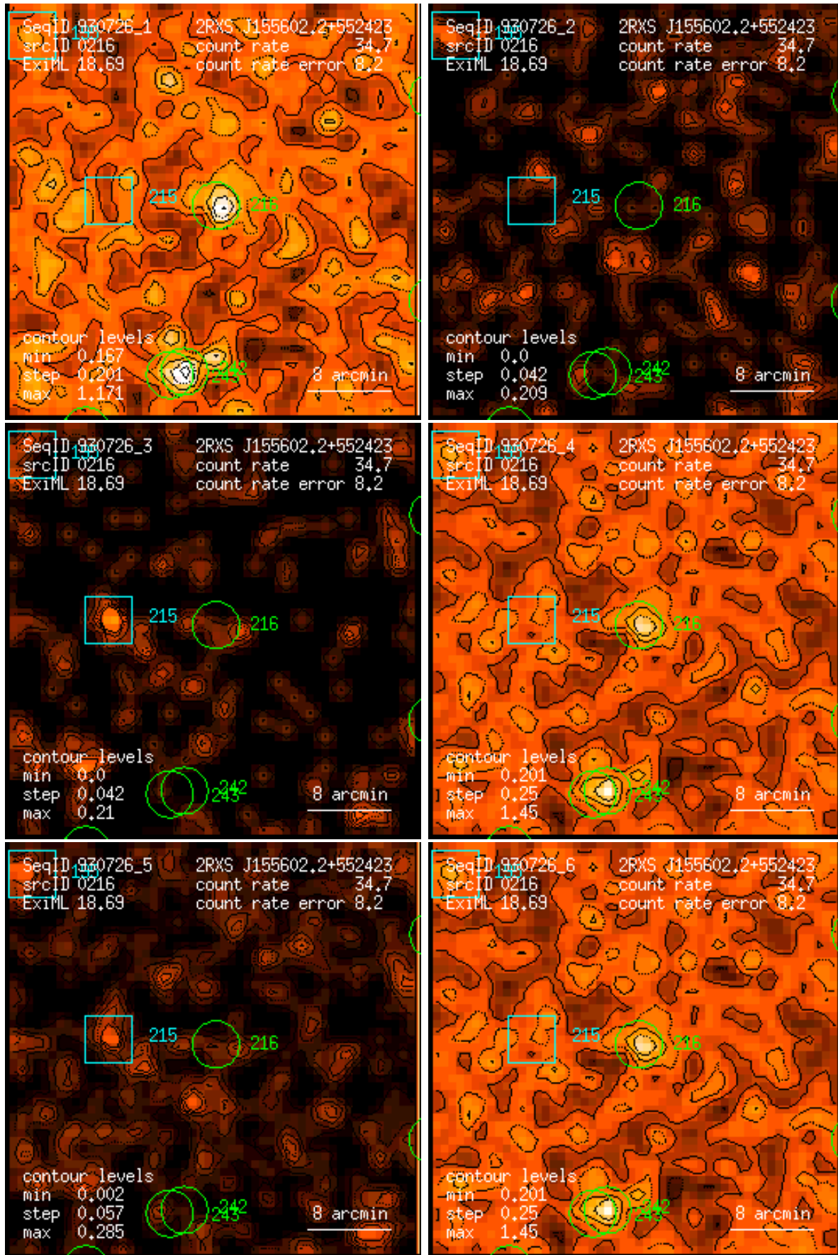
Figure 216: RASS 930726: detection 0216: band rate images, Gaussian filter: (1) PSPC channels 11 – 41, (2) 52 – 90, (3) 91 – 201, (4) 11 – 235, (5) 52 – 201, (6) 11 – 201. Broad band rates in counts/ks. Band rate contour levels in counts/ks/arcmin 2 .
