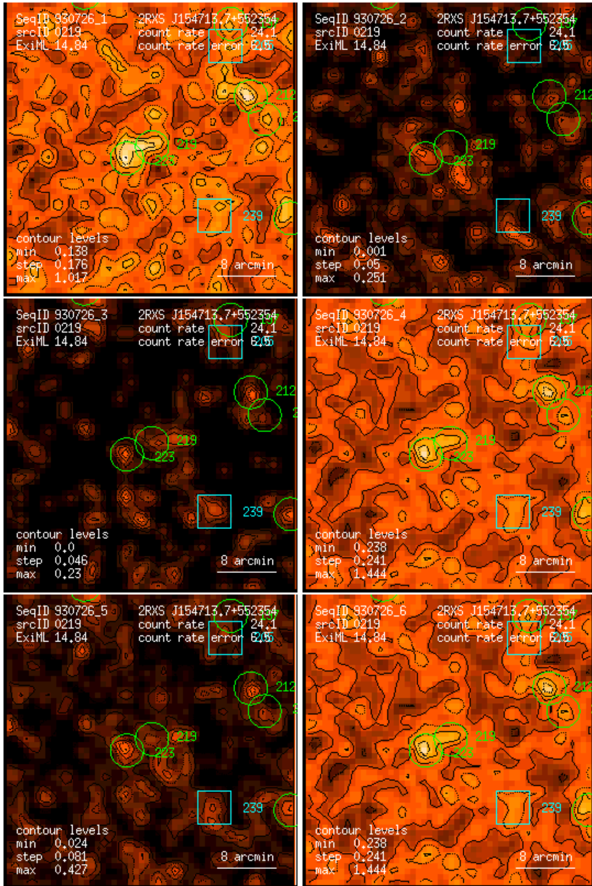
Figure 219: RASS 930726: detection 0219: band rate images, Gaussian filter: (1) PSPC channels 11 – 41, (2) 52 – 90, (3) 91 – 201, (4) 11 – 235, (5) 52 – 201, (6) 11 – 201. Broad band rates in counts/ks. Band rate contour levels in counts/ks/arcmin 2 .
