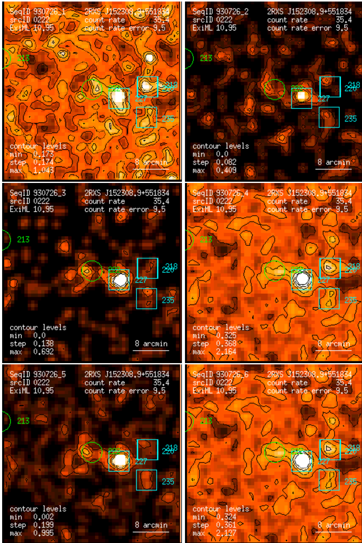
Figure 222: RASS 930726: detection 0222: band rate images, Gaussian filter: (1) PSPC channels 11 – 41, (2) 52 – 90, (3) 91 – 201, (4) 11 – 235, (5) 52 – 201, (6) 11 – 201. Broad band rates in counts/ks. Band rate contour levels in counts/ks/arcmin 2 .
