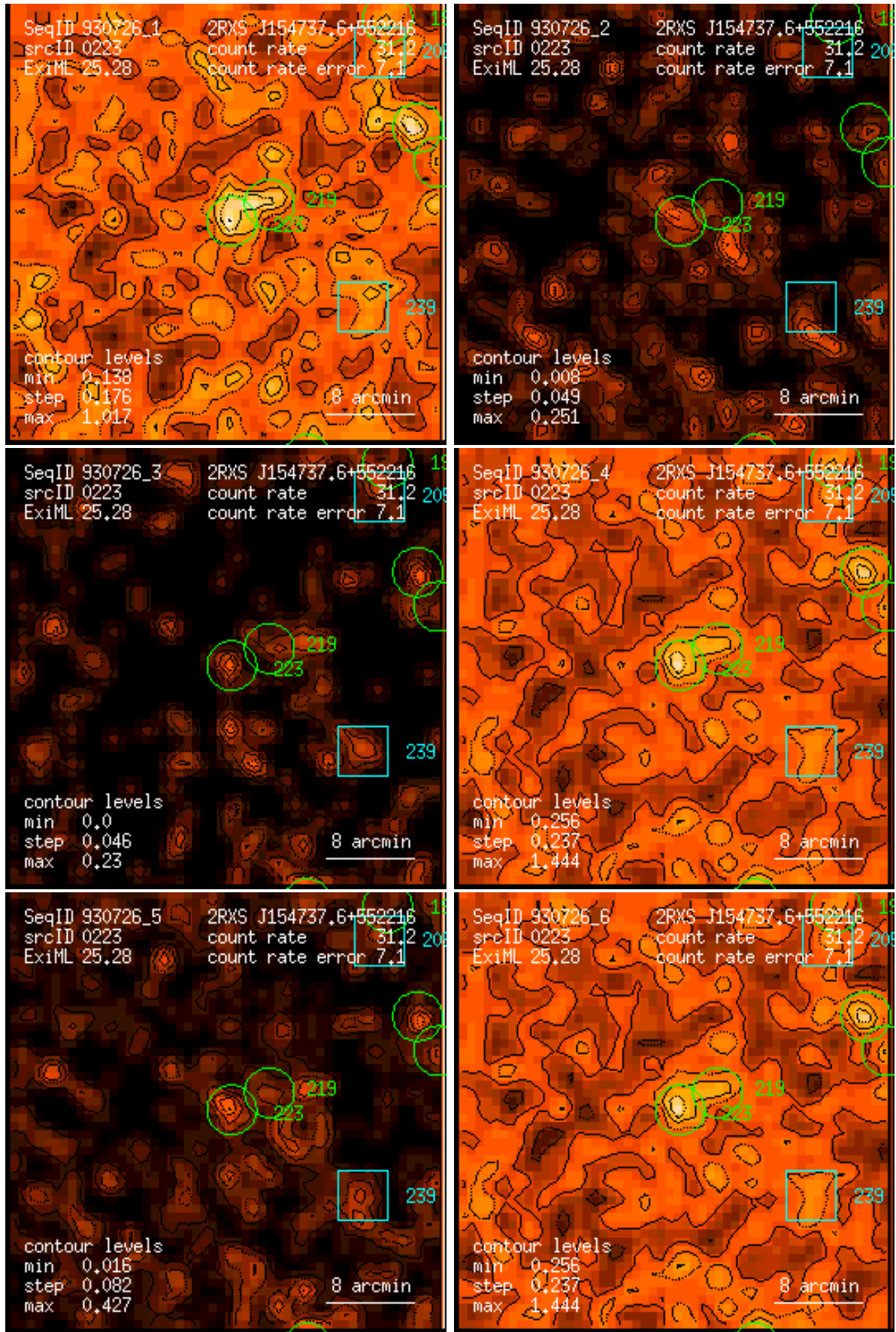
Figure 223: RASS 930726: detection 0223: band rate images, Gaussian filter: (1) PSPC channels 11 – 41, (2) 52 – 90, (3) 91 – 201, (4) 11 – 235, (5) 52 – 201, (6) 11 – 201. Broad band rates in counts/ks. Band rate contour levels in counts/ks/arcmin 2 .
