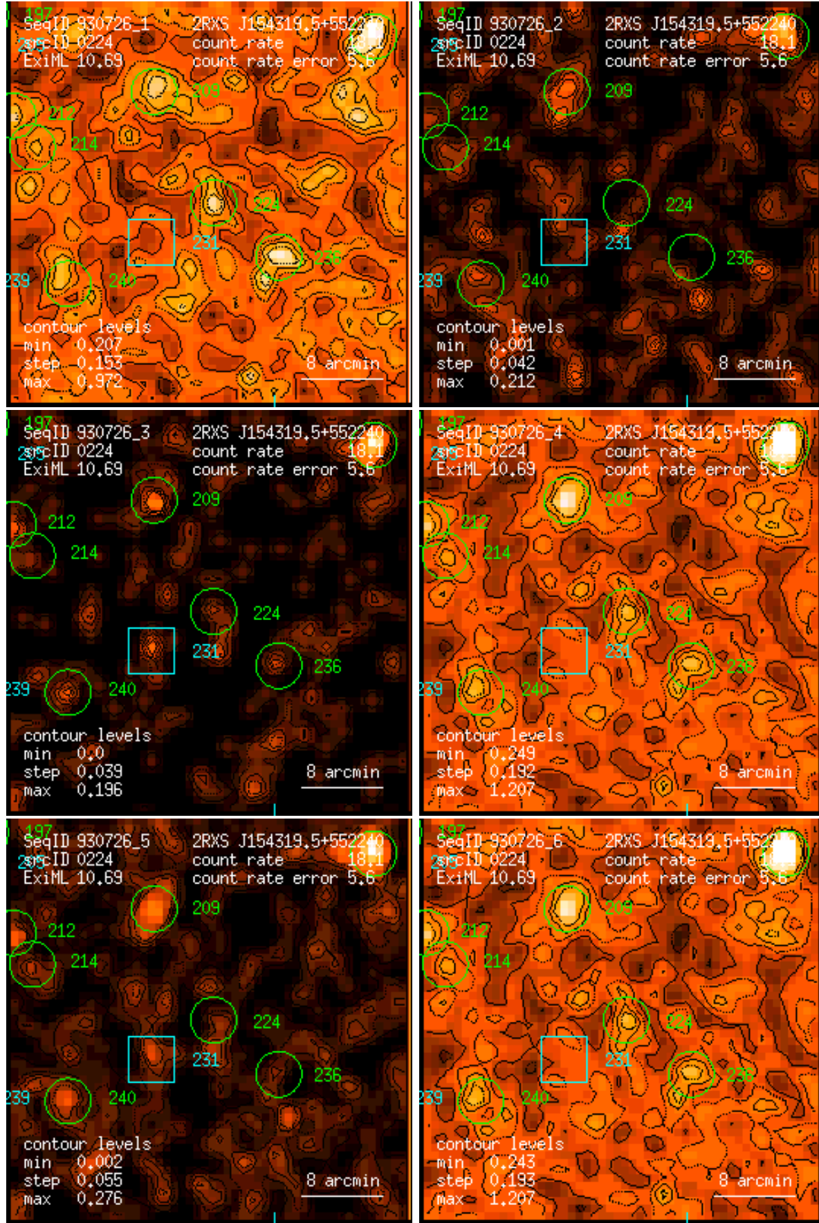
Figure 224: RASS 930726: detection 0224: band rate images, Gaussian filter: (1) PSPC channels 11 – 41, (2) 52 – 90, (3) 91 – 201, (4) 11 – 235, (5) 52 – 201, (6) 11 – 201. Broad band rates in counts/ks. Band rate contour levels in counts/ks/arcmin 2 .
