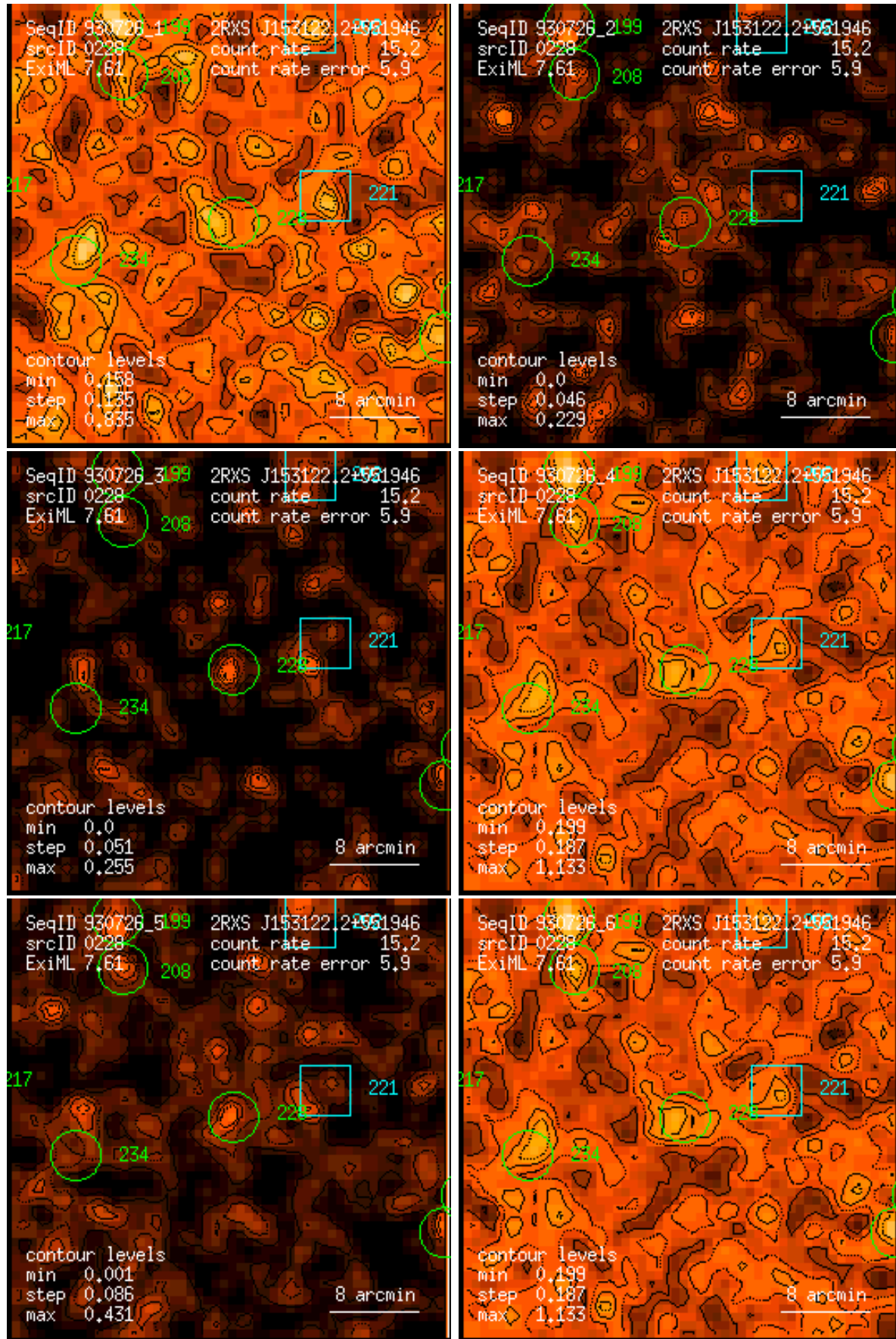
Figure 228: RASS 930726: detection 0228: band rate images, Gaussian filter: (1) PSPC channels 11 – 41, (2) 52 – 90, (3) 91 – 201, (4) 11 – 235, (5) 52 – 201, (6) 11 – 201. Broad band rates in counts/ks. Band rate contour levels in counts/ks/arcmin 2 .
