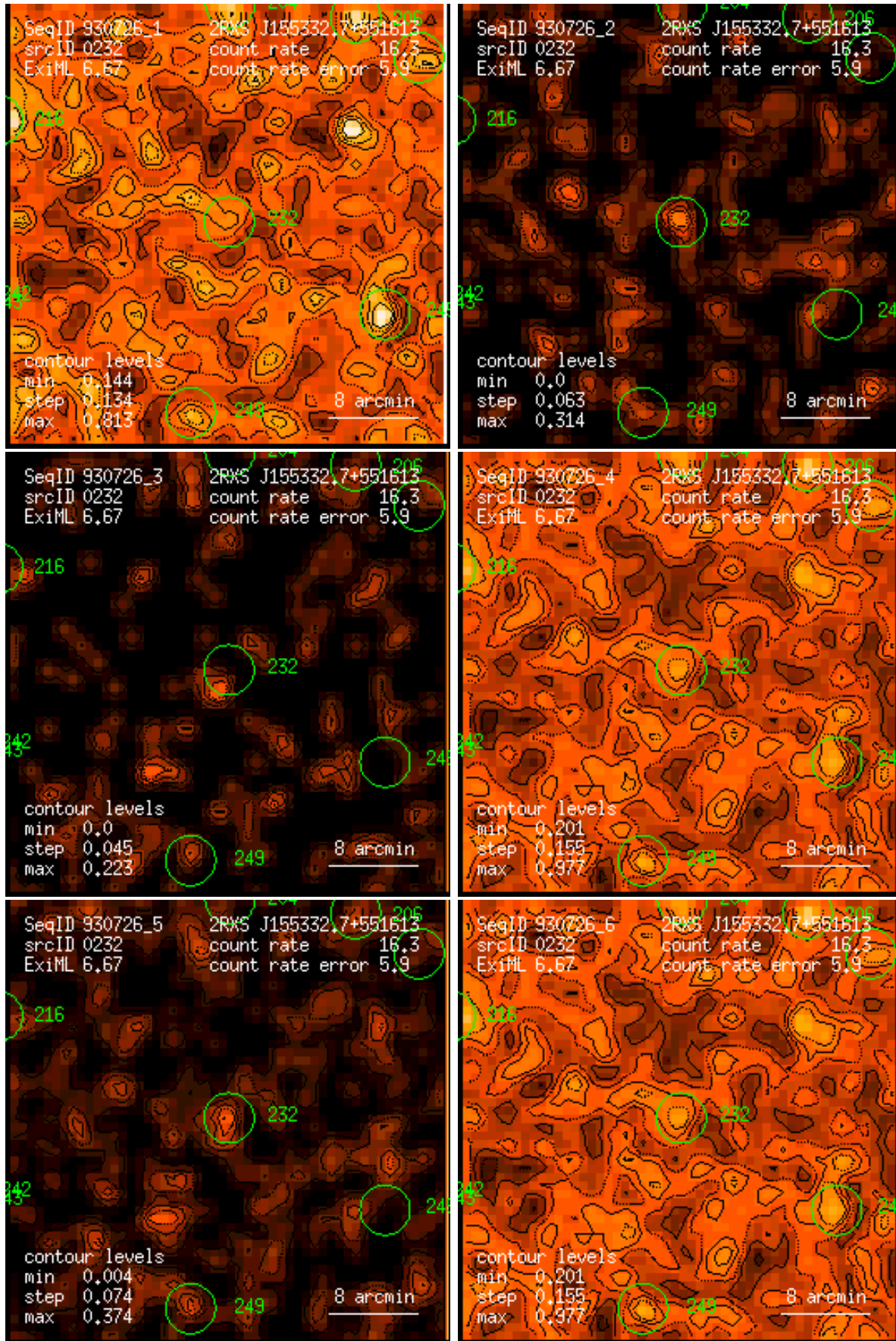
Figure 232: RASS 930726: detection 0232: band rate images, Gaussian filter: (1) PSPC channels 11 – 41, (2) 52 – 90, (3) 91 – 201, (4) 11 – 235, (5) 52 – 201, (6) 11 – 201. Broad band rates in counts/ks. Band rate contour levels in counts/ks/arcmin 2 .
