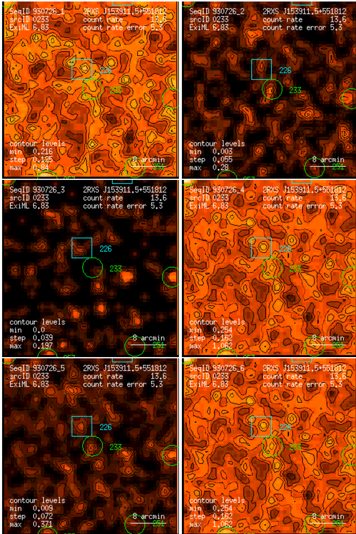
Figure 233: RASS 930726: detection 0233: band rate images, Gaussian filter: (1) PSPC channels 11 – 41, (2) 52 – 90, (3) 91 – 201, (4) 11 – 235, (5) 52 – 201, (6) 11 – 201. Broad band rates in counts/ks. Band rate contour levels in counts/ks/arcmin 2 .
