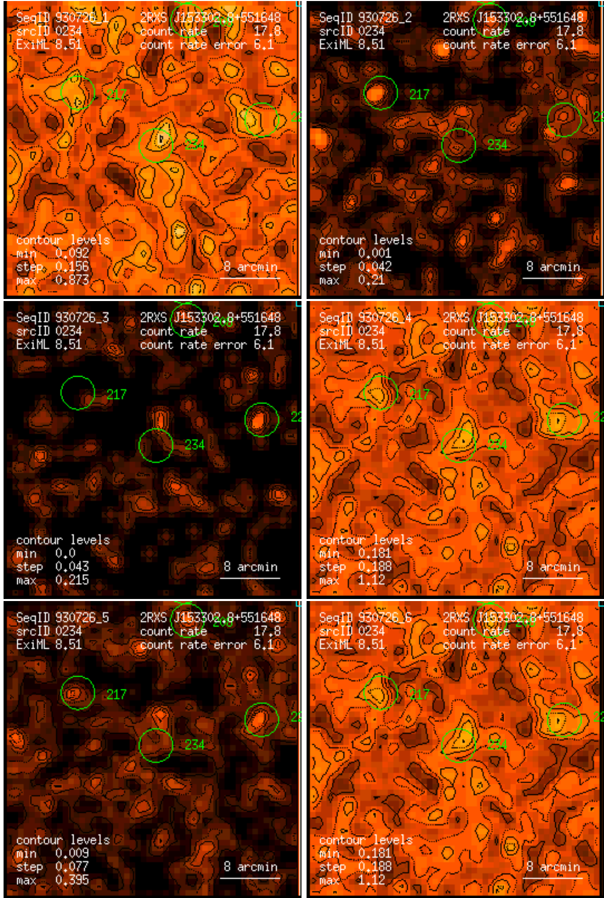
Figure 234: RASS 930726: detection 0234: band rate images, Gaussian filter: (1) PSPC channels 11 – 41, (2) 52 – 90, (3) 91 – 201, (4) 11 – 235, (5) 52 – 201, (6) 11 – 201. Broad band rates in counts/ks. Band rate contour levels in counts/ks/arcmin 2 .
