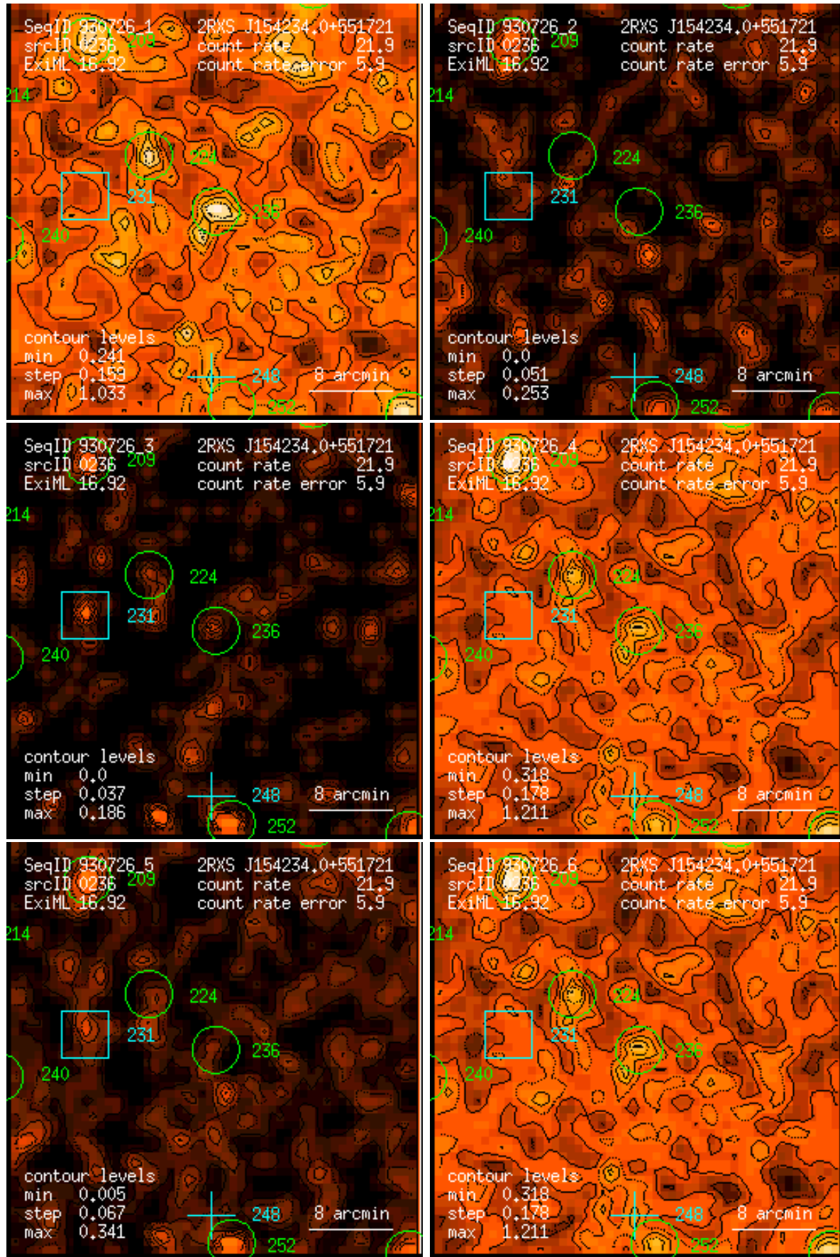
Figure 236: RASS 930726: detection 0236: band rate images, Gaussian filter: (1) PSPC channels 11 – 41, (2) 52 – 90, (3) 91 – 201, (4) 11 – 235, (5) 52 – 201, (6) 11 – 201. Broad band rates in counts/ks. Band rate contour levels in counts/ks/arcmin 2 .
