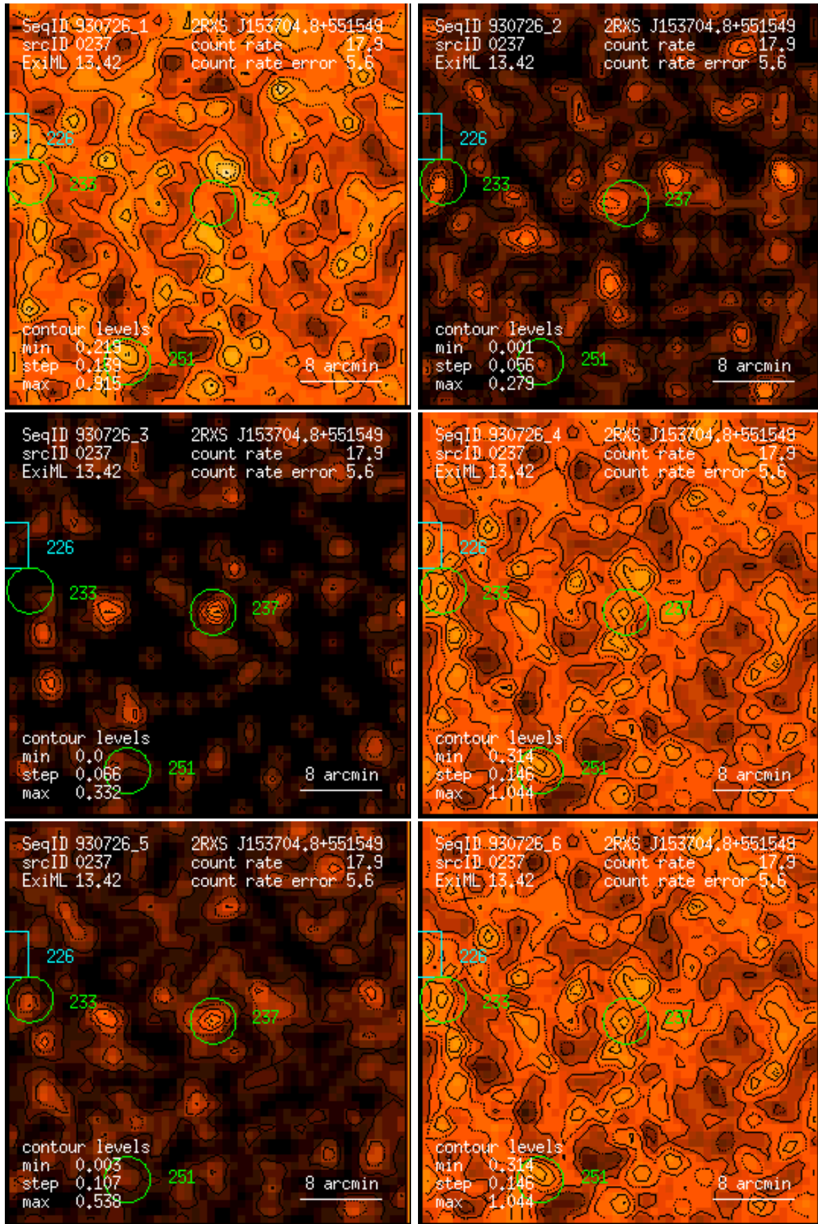
Figure 237: RASS 930726: detection 0237: band rate images, Gaussian filter: (1) PSPC channels 11 – 41, (2) 52 – 90, (3) 91 – 201, (4) 11 – 235, (5) 52 – 201, (6) 11 – 201. Broad band rates in counts/ks. Band rate contour levels in counts/ks/arcmin 2 .
