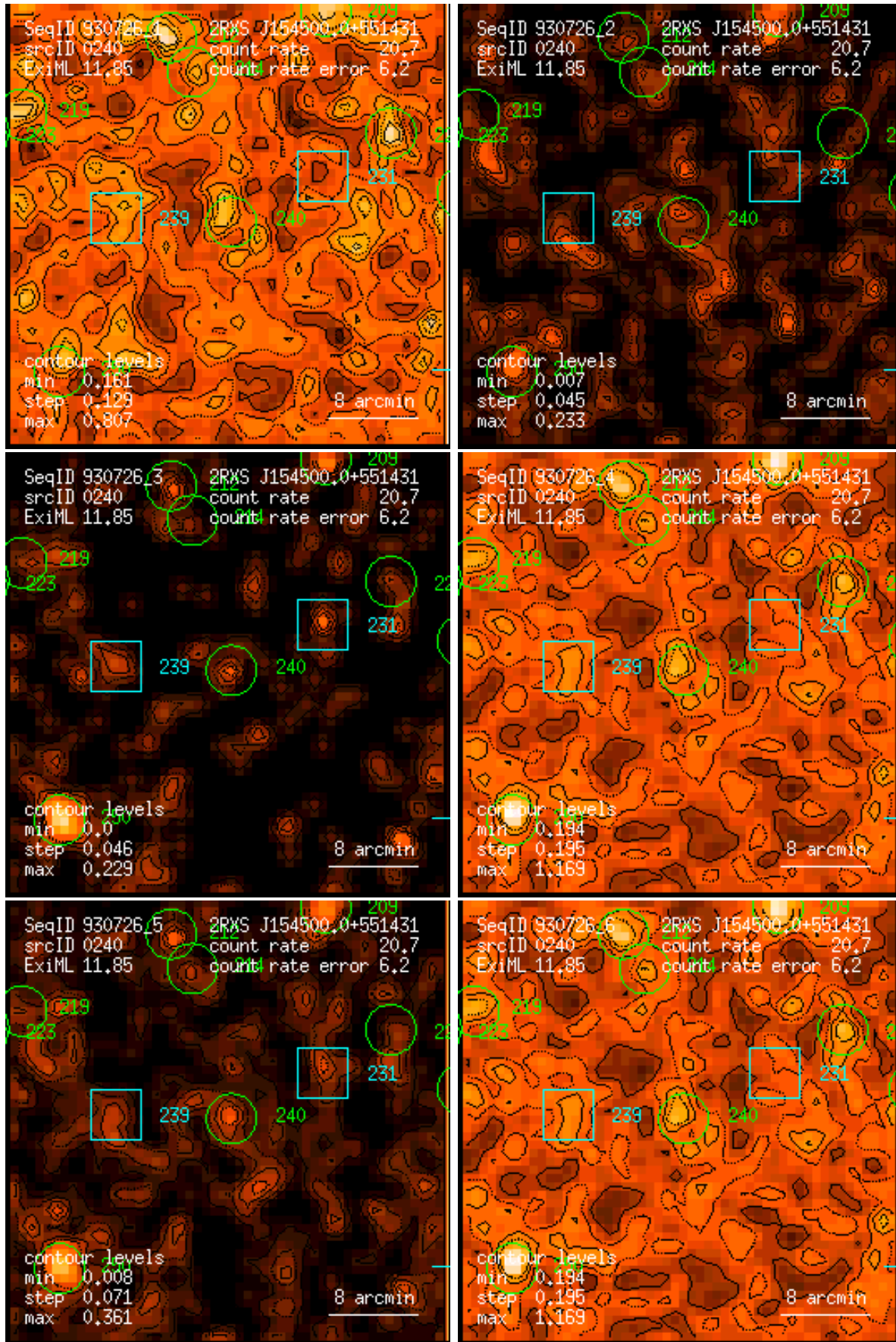
Figure 240: RASS 930726: detection 0240: band rate images, Gaussian filter: (1) PSPC channels 11 – 41, (2) 52 – 90, (3) 91 – 201, (4) 11 – 235, (5) 52 – 201, (6) 11 – 201. Broad band rates in counts/ks. Band rate contour levels in counts/ks/arcmin 2 .
