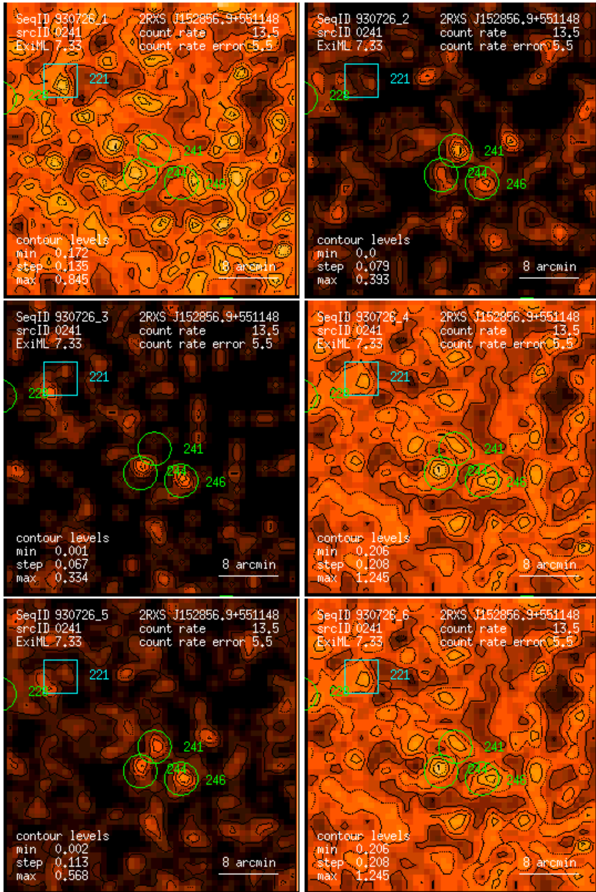
Figure 241: RASS 930726: detection 0241: band rate images, Gaussian filter: (1) PSPC channels 11 – 41, (2) 52 – 90, (3) 91 – 201, (4) 11 – 235, (5) 52 – 201, (6) 11 – 201. Broad band rates in counts/ks. Band rate contour levels in counts/ks/arcmin 2 .
