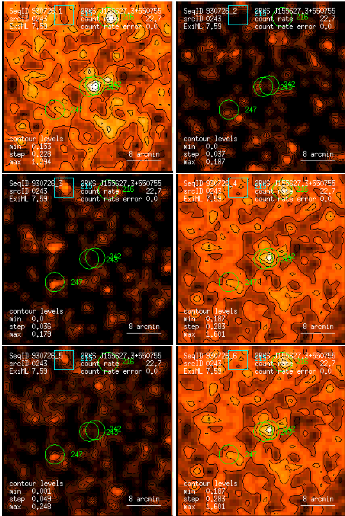
Figure 243: RASS 930726: detection 0243: band rate images, Gaussian filter: (1) PSPC channels 11 – 41, (2) 52 – 90, (3) 91 – 201, (4) 11 – 235, (5) 52 – 201, (6) 11 – 201. Broad band rates in counts/ks. Band rate contour levels in counts/ks/arcmin 2 .
