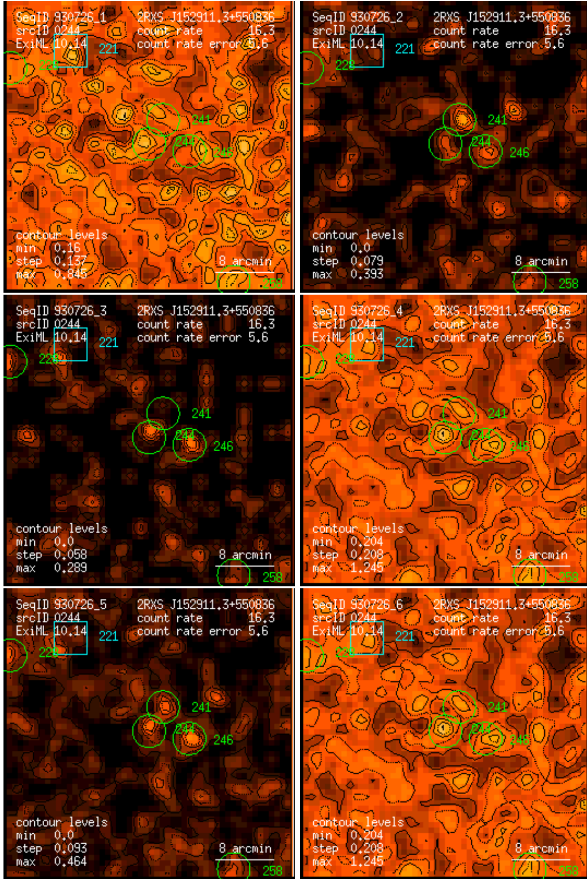
Figure 244: RASS 930726: detection 0244: band rate images, Gaussian filter: (1) PSPC channels 11 – 41, (2) 52 – 90, (3) 91 – 201, (4) 11 – 235, (5) 52 – 201, (6) 11 – 201. Broad band rates in counts/ks. Band rate contour levels in counts/ks/arcmin 2 .
