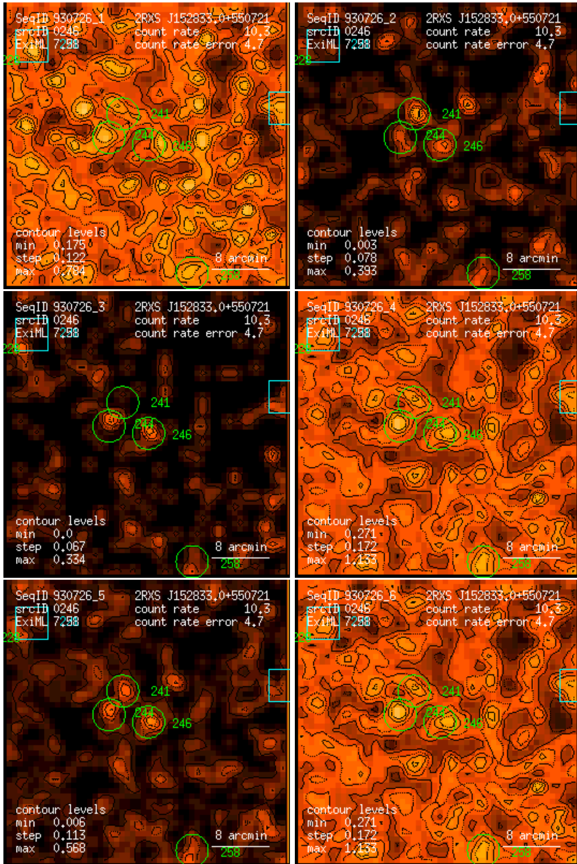
Figure 246: RASS 930726: detection 0246: band rate images, Gaussian filter: (1) PSPC channels 11 – 41, (2) 52 – 90, (3) 91 – 201, (4) 11 – 235, (5) 52 – 201, (6) 11 – 201. Broad band rates in counts/ks. Band rate contour levels in counts/ks/arcmin 2 .
