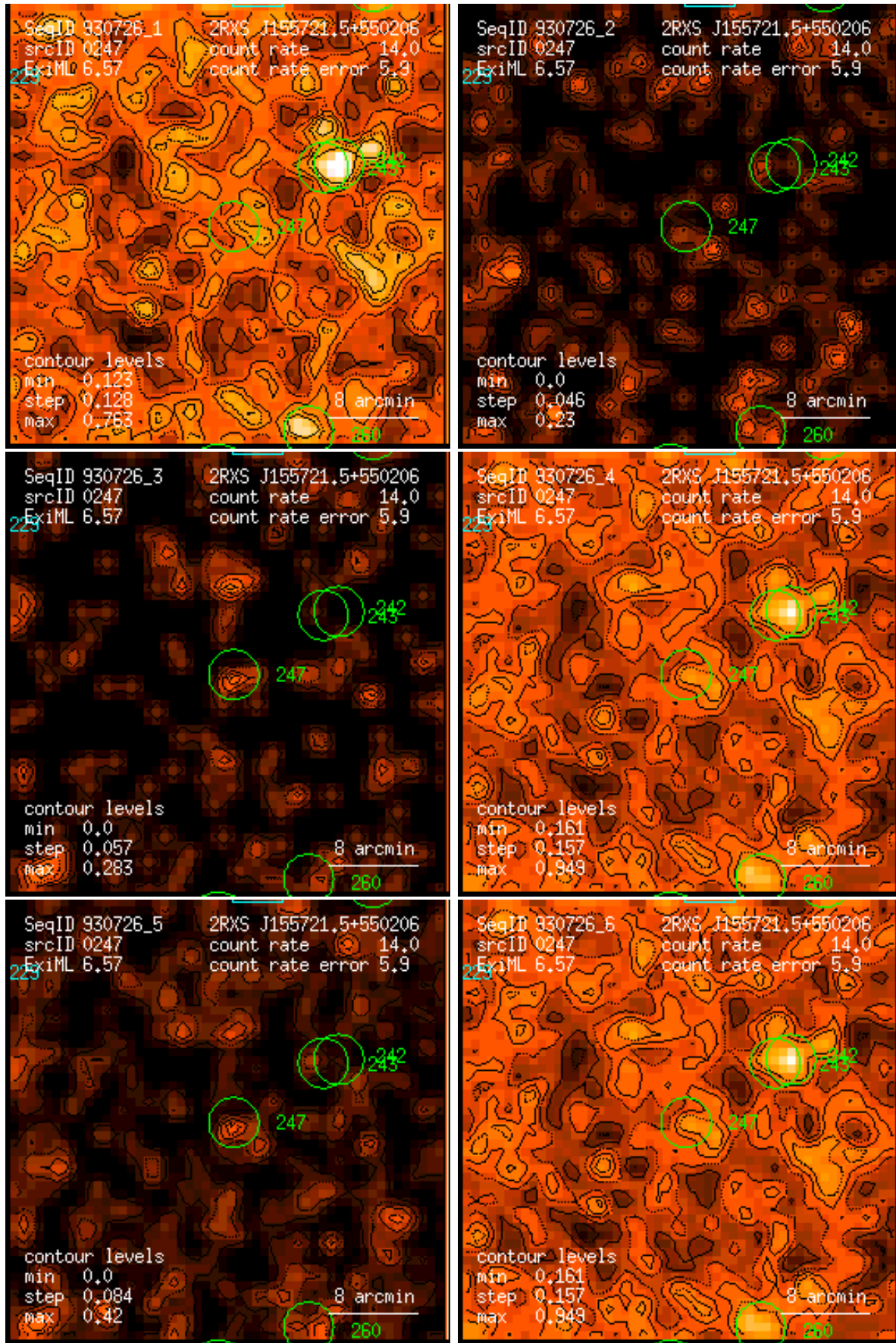
Figure 247: RASS 930726: detection 0247: band rate images, Gaussian filter: (1) PSPC channels 11 – 41, (2) 52 – 90, (3) 91 – 201, (4) 11 – 235, (5) 52 – 201, (6) 11 – 201. Broad band rates in counts/ks. Band rate contour levels in counts/ks/arcmin 2 .
