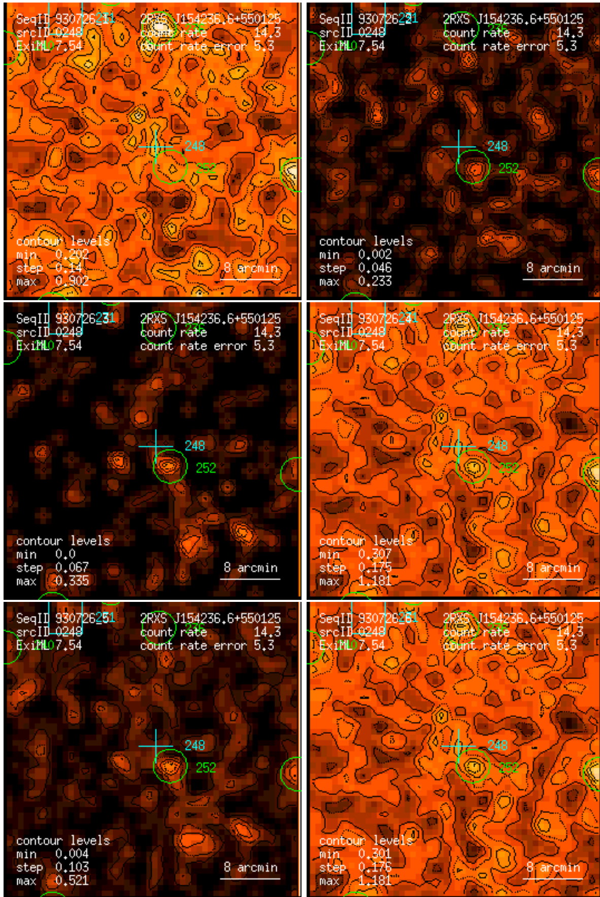
Figure 248: RASS 930726: detection 0248: band rate images, Gaussian filter: (1) PSPC channels 11 – 41, (2) 52 – 90, (3) 91 – 201, (4) 11 – 235, (5) 52 – 201, (6) 11 – 201. Broad band rates in counts/ks. Band rate contour levels in counts/ks/arcmin 2 .
