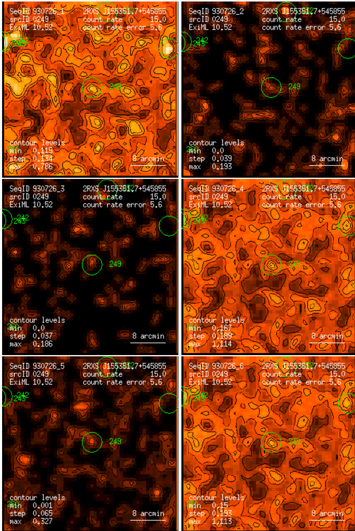
Figure 249: RASS 930726: detection 0249: band rate images, Gaussian filter: (1) PSPC channels 11 – 41, (2) 52 – 90, (3) 91 – 201, (4) 11 – 235, (5) 52 – 201, (6) 11 – 201. Broad band rates in counts/ks. Band rate contour levels in counts/ks/arcmin 2 .
