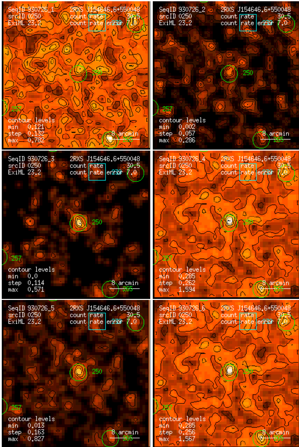
Figure 250: RASS 930726: detection 0250: band rate images, Gaussian filter: (1) PSPC channels 11 – 41, (2) 52 – 90, (3) 91 – 201, (4) 11 – 235, (5) 52 – 201, (6) 11 – 201. Broad band rates in counts/ks. Band rate contour levels in counts/ks/arcmin 2 .
