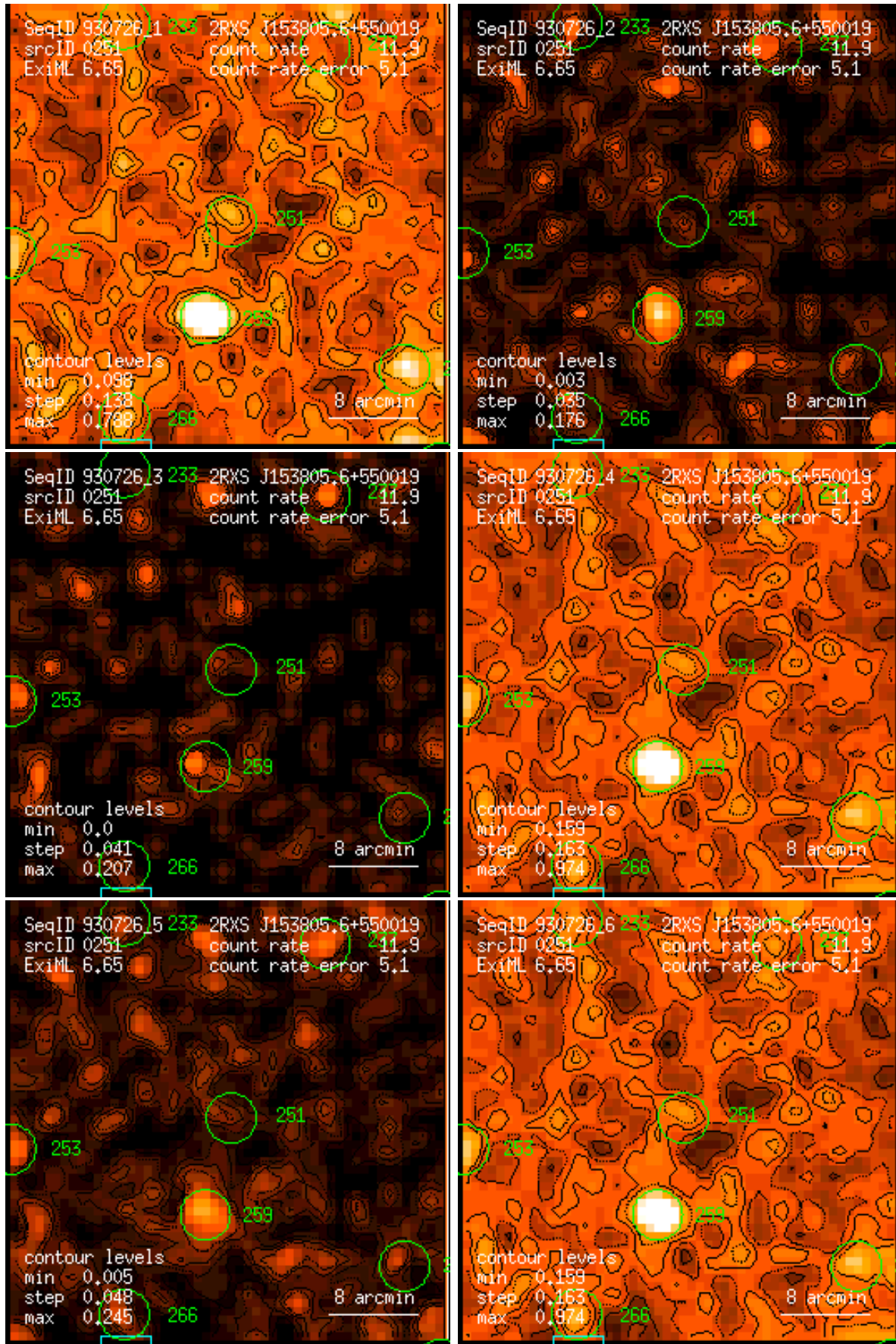
Figure 251: RASS 930726: detection 0251: band rate images, Gaussian filter: (1) PSPC channels 11 – 41, (2) 52 – 90, (3) 91 – 201, (4) 11 – 235, (5) 52 – 201, (6) 11 – 201. Broad band rates in counts/ks. Band rate contour levels in counts/ks/arcmin 2 .
