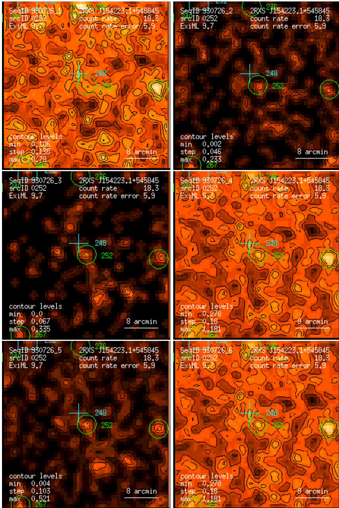
Figure 252: RASS 930726: detection 0252: band rate images, Gaussian filter: (1) PSPC channels 11 – 41, (2) 52 – 90, (3) 91 – 201, (4) 11 – 235, (5) 52 – 201, (6) 11 – 201. Broad band rates in counts/ks. Band rate contour levels in counts/ks/arcmin 2 .
