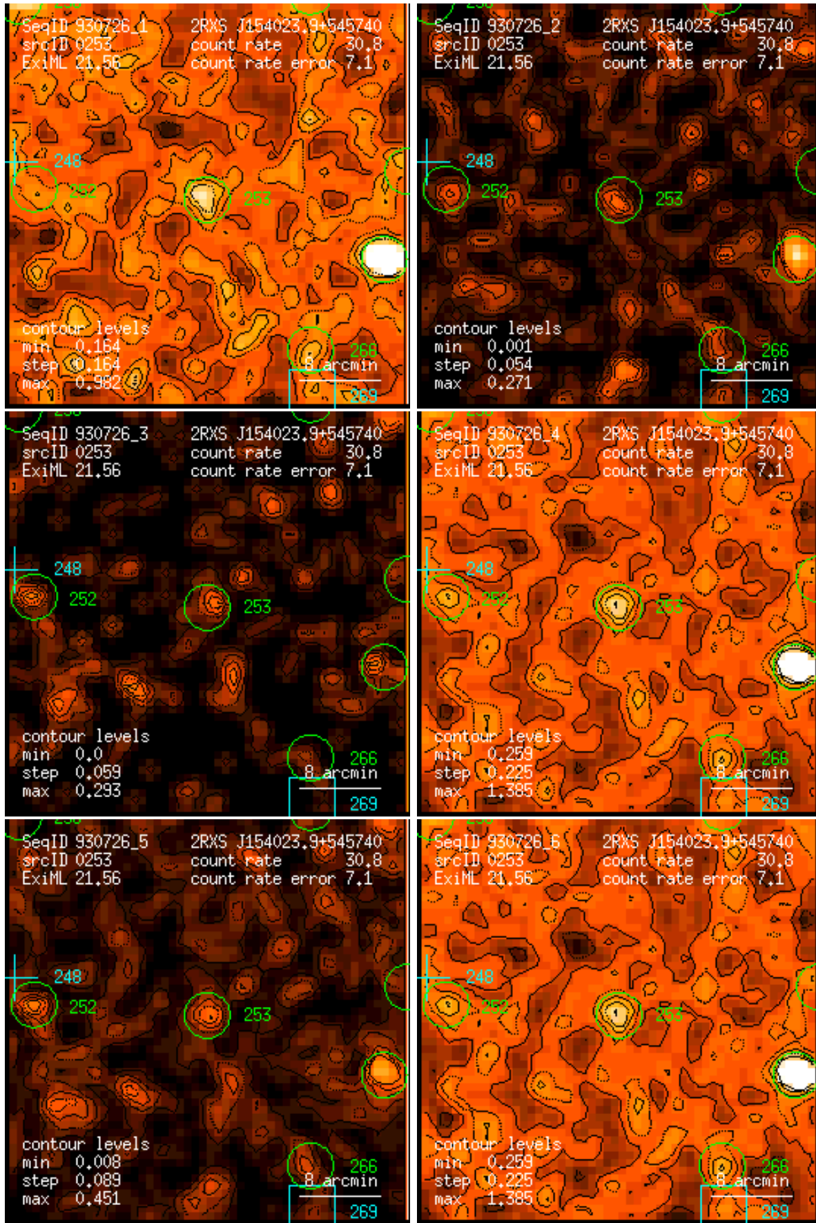
Figure 253: RASS 930726: detection 0253: band rate images, Gaussian filter: (1) PSPC channels 11 – 41, (2) 52 – 90, (3) 91 – 201, (4) 11 – 235, (5) 52 – 201, (6) 11 – 201. Broad band rates in counts/ks. Band rate contour levels in counts/ks/arcmin 2 .
