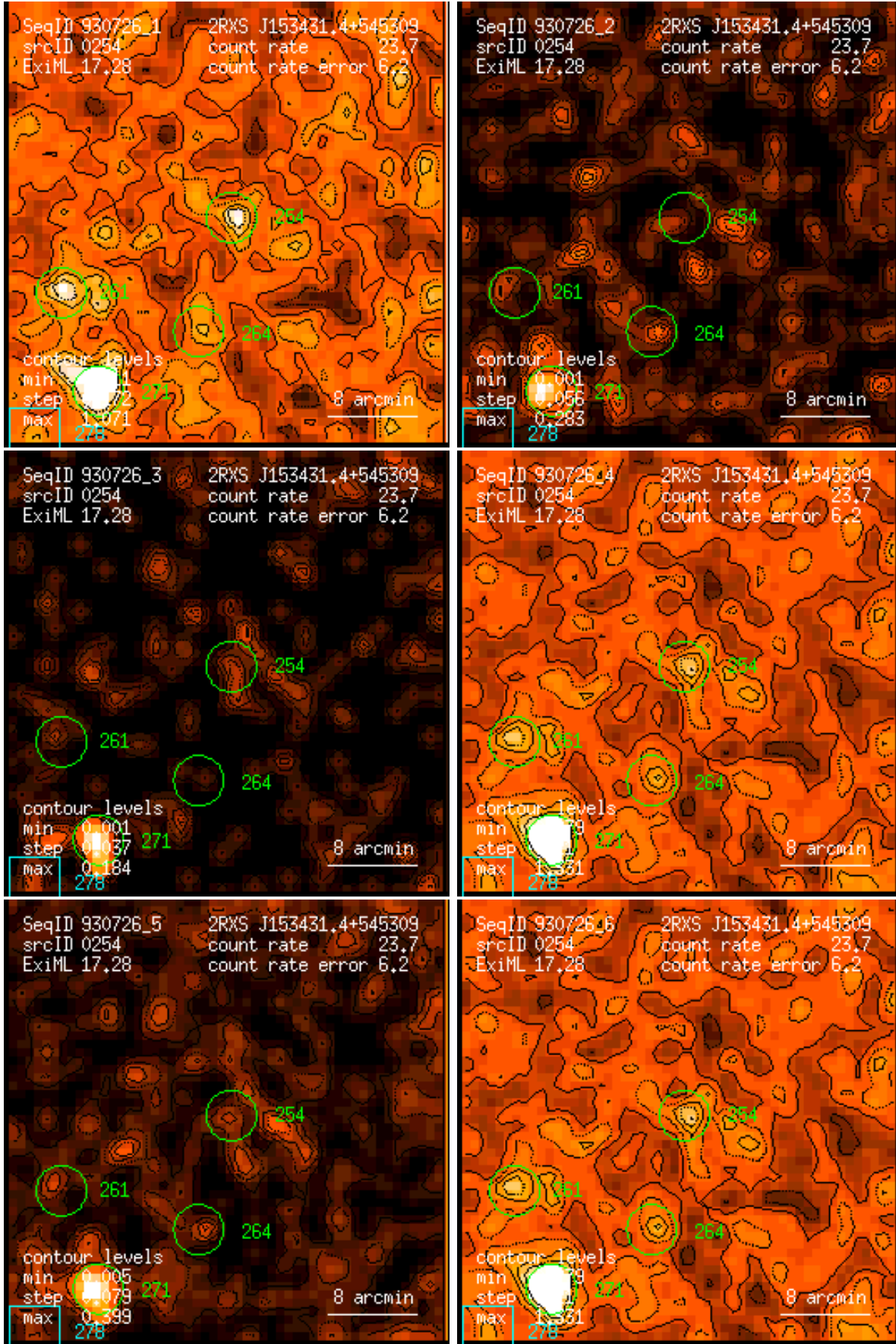
Figure 254: RASS 930726: detection 0254: band rate images, Gaussian filter: (1) PSPC channels 11 – 41, (2) 52 – 90, (3) 91 – 201, (4) 11 – 235, (5) 52 – 201, (6) 11 – 201. Broad band rates in counts/ks. Band rate contour levels in counts/ks/arcmin 2 .
