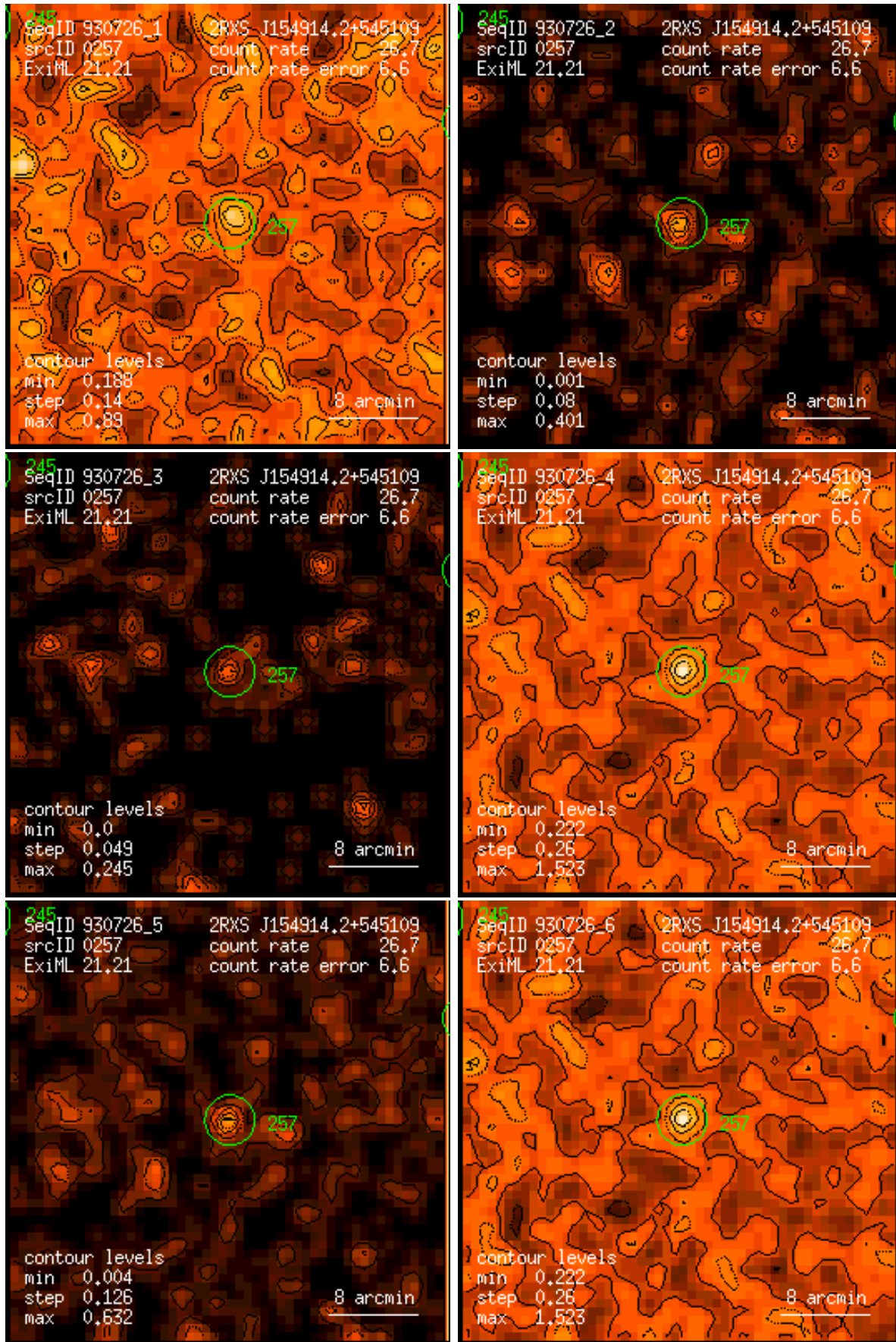
Figure 257: RASS 930726: detection 0257: band rate images, Gaussian filter: (1) PSPC channels 11 – 41, (2) 52 – 90, (3) 91 – 201, (4) 11 – 235, (5) 52 – 201, (6) 11 – 201. Broad band rates in counts/ks. Band rate contour levels in counts/ks/arcmin 2 .
