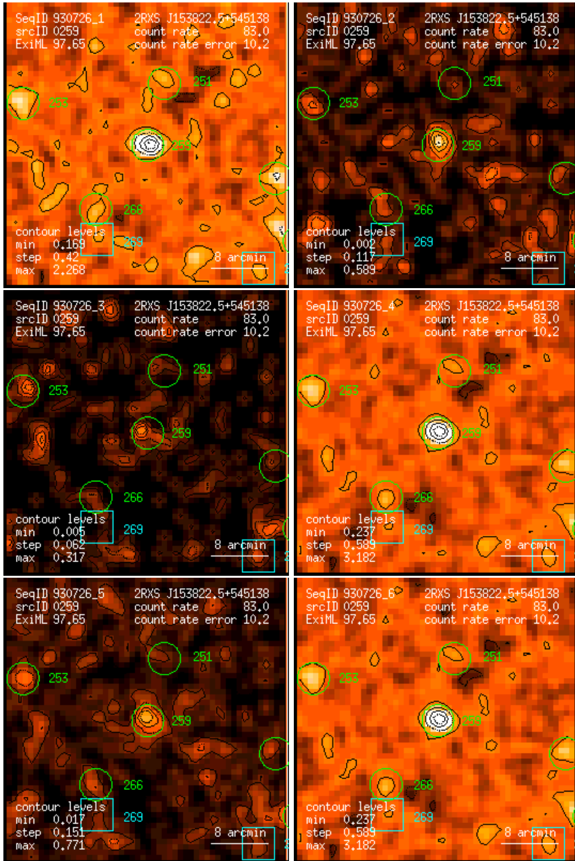
Figure 259: RASS 930726: detection 0259: band rate images, Gaussian filter: (1) PSPC channels 11 – 41, (2) 52 – 90, (3) 91 – 201, (4) 11 – 235, (5) 52 – 201, (6) 11 – 201. Broad band rates in counts/ks. Band rate contour levels in counts/ks/arcmin 2 .
