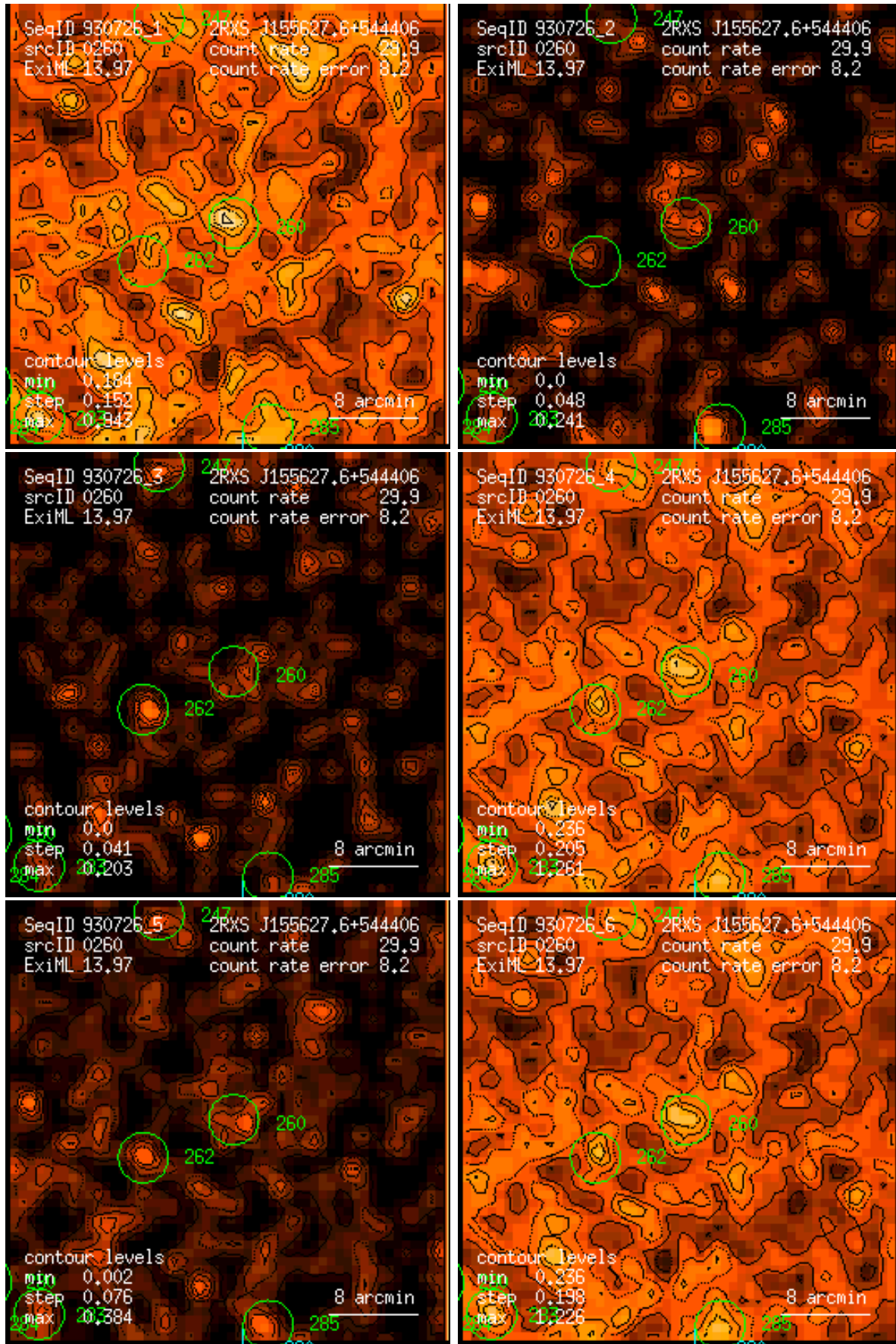
Figure 260: RASS 930726: detection 0260: band rate images, Gaussian filter: (1) PSPPC channels 11 – 41, (2) 52 – 90, (3) 91 – 201, (4) 11 – 235, (5) 52 – 201, (6) 11 – 201. Broad band rates in counts/ks. Band rate contour levels in counts/ks/arcmin 2 .
