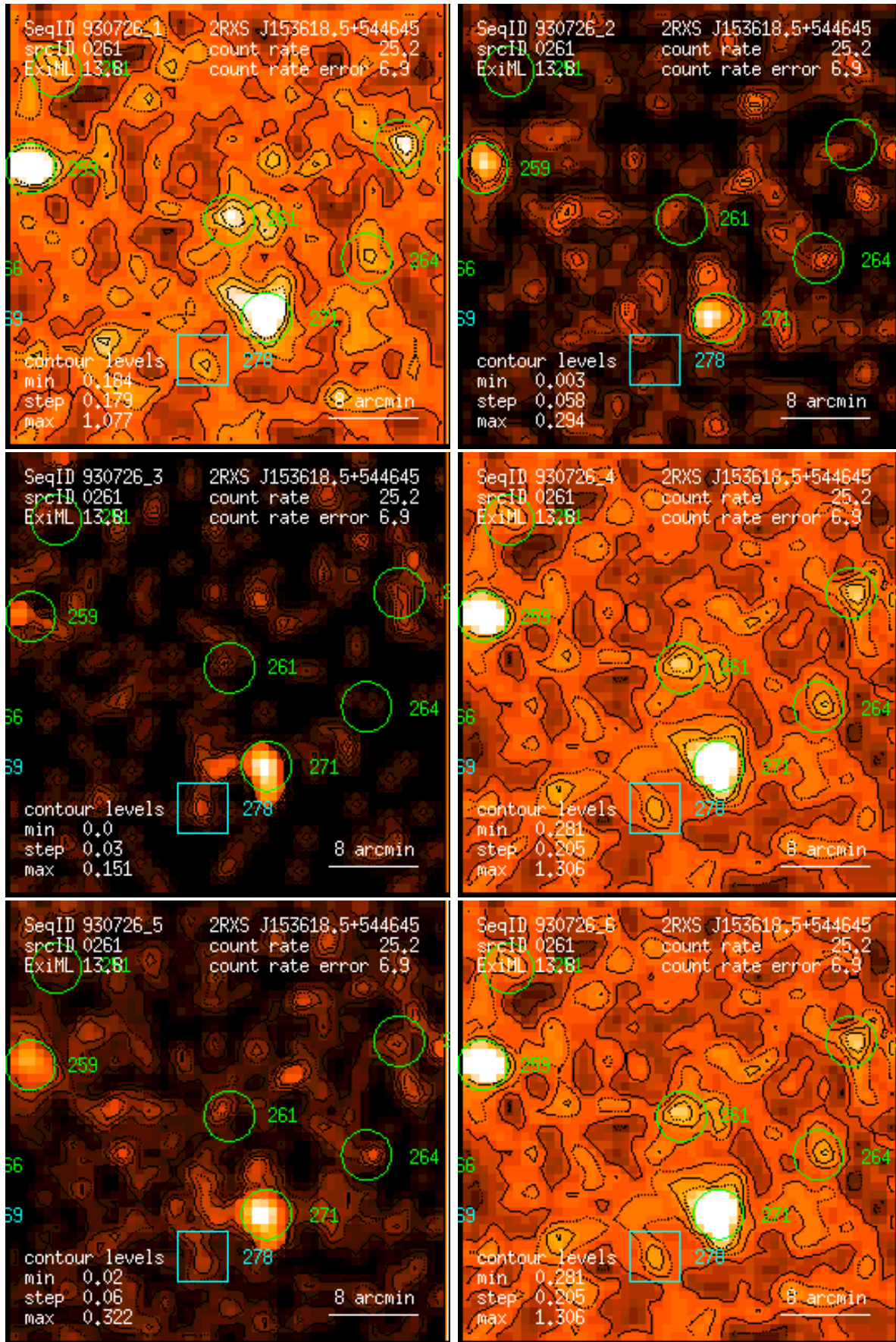
Figure 261: RASS 930726: detection 0261: band rate images, Gaussian filter: (1) PSPC channels 11 – 41, (2) 52 – 90, (3) 91 – 201, (4) 11 – 235, (5) 52 – 201, (6) 11 – 201. Broad band rates in counts/ks. Band rate contour levels in counts/ks/arcmin 2 .
