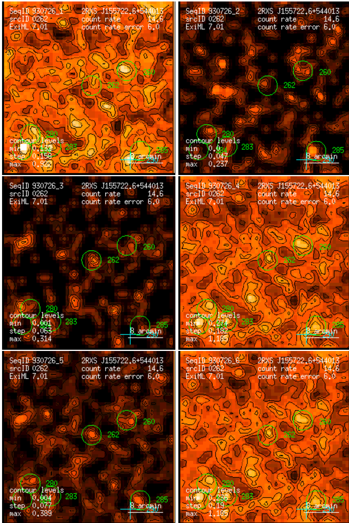
Figure 262: RASS 930726: detection 0262: band rate images, Gaussian filter: (1) PSPC channels 11 – 41, (2) 52 – 90, (3) 91 – 201, (4) 11 – 235, (5) 52 – 201, (6) 11 – 201. Broad band rates in counts/ks. Band rate contour levels in counts/ks/arcmin 2 .
