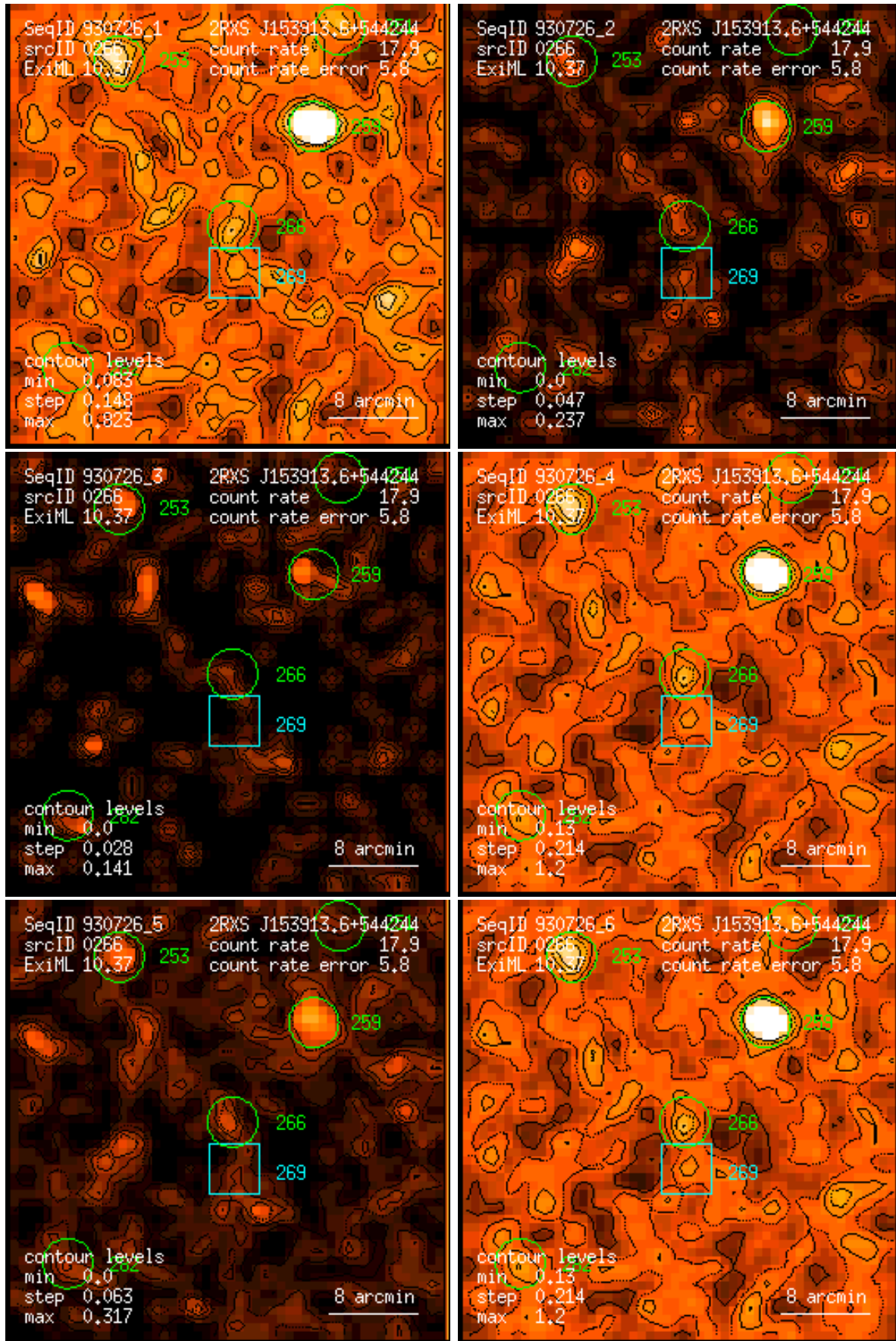
Figure 266: RASS 930726: detection 0266: band rate images, Gaussian filter: (1) PSPC channels 11 – 41, (2) 52 – 90, (3) 91 – 201, (4) 11 – 235, (5) 52 – 201, (6) 11 – 201. Broad band rates in counts/ks. Band rate contour levels in counts/ks/arcmin 2 .
