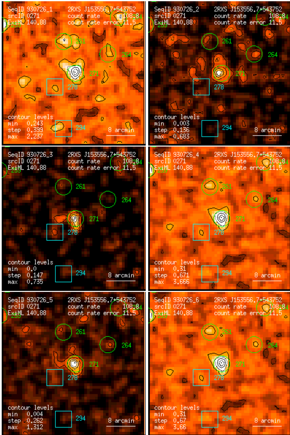
Figure 271: RASS 930726: detection 0271: band rate images, Gaussian filter: (1) PSPC channels 11 – 41, (2) 52 – 90, (3) 91 – 201, (4) 11 – 235, (5) 52 – 201, (6) 11 – 201. Broad band rates in counts/ks. Band rate contour levels in counts/ks/arcmin 2 .
