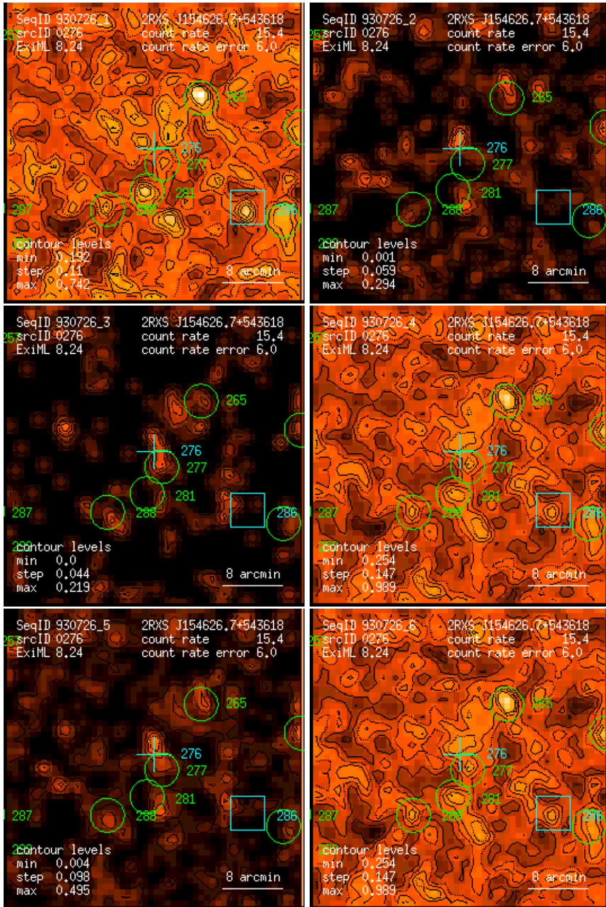
Figure 276: RASS 930726: detection 0276: band rate images, Gaussian filter: (1) PSPC channels 11 – 41, (2) 52 – 90, (3) 91 – 201, (4) 11 – 235, (5) 52 – 201, (6) 11 – 201. Broad band rates in counts/ks. Band rate contour levels in counts/ks/arcmin 2 .
