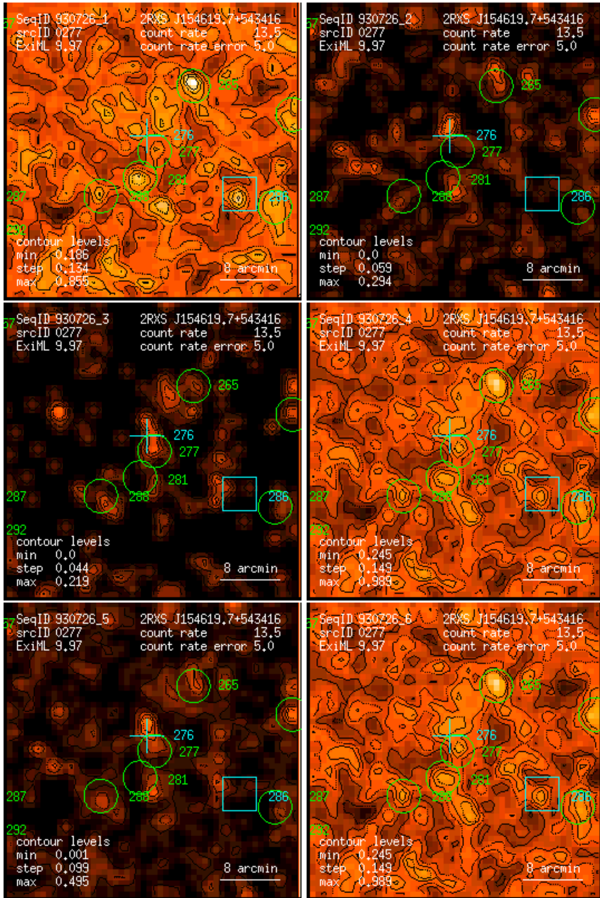
Figure 277: RASS 930726: detection 0277: band rate images, Gaussian filter: (1) PSPC channels 11 – 41, (2) 52 – 90, (3) 91 – 201, (4) 11 – 235, (5) 52 – 201, (6) 11 – 201. Broad band rates in counts/ks. Band rate contour levels in counts/ks/arcmin 2 .
