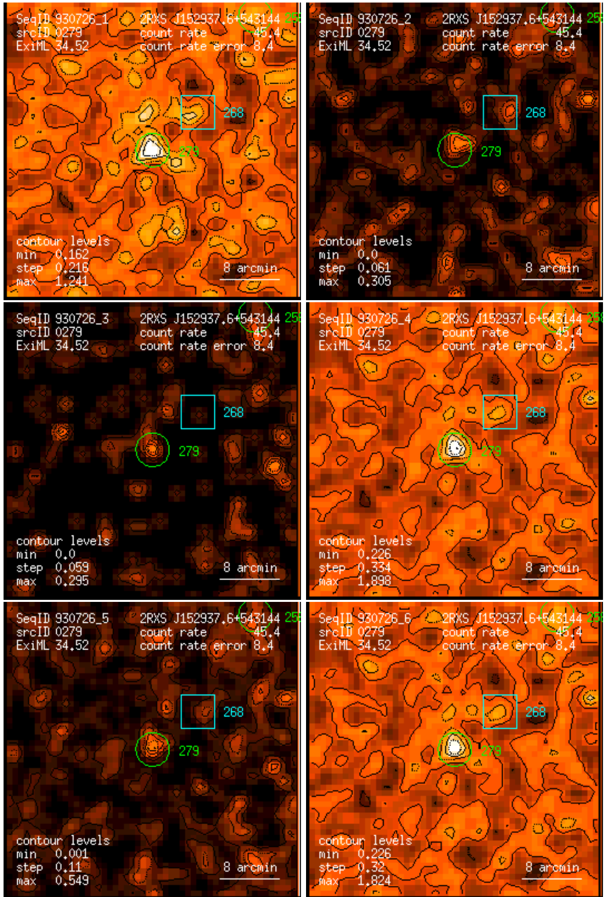
Figure 279: RASS 930726: detection 0279: band rate images, Gaussian filter: (1) PSPC channels 11 – 41, (2) 52 – 90, (3) 91 – 201, (4) 11 – 235, (5) 52 – 201, (6) 11 – 201. Broad band rates in counts/ks. Band rate contour levels in counts/ks/arcmin 2 .
