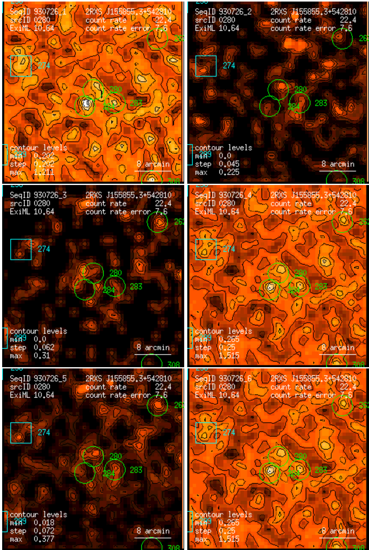
Figure 280: RASS 930726: detection 0280: band rate images, Gaussian filter: (1) PSPC channels 11 – 41, (2) 52 – 90, (3) 91 – 201, (4) 11 – 235, (5) 52 – 201, (6) 11 – 201. Broad band rates in counts/ks. Band rate contour levels in counts/ks/arcmin 2 .
