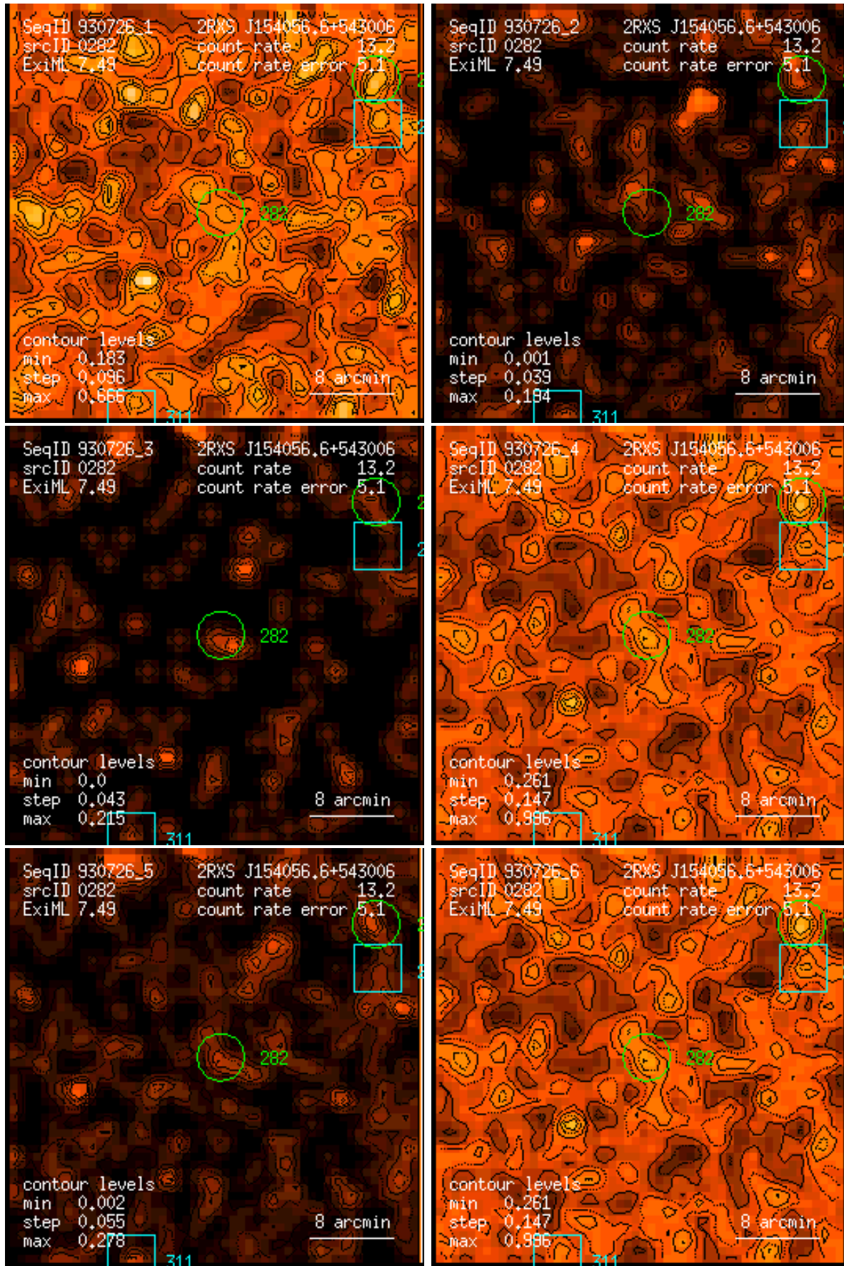
Figure 282: RASS 930726: detection 0282: band rate images, Gaussian filter: (1) PSPC channels 11 – 41, (2) 52 – 90, (3) 91 – 201, (4) 11 – 235, (5) 52 – 201, (6) 11 – 201. Broad band rates in counts/ks. Band rate contour levels in counts/ks/arcmin 2 .
