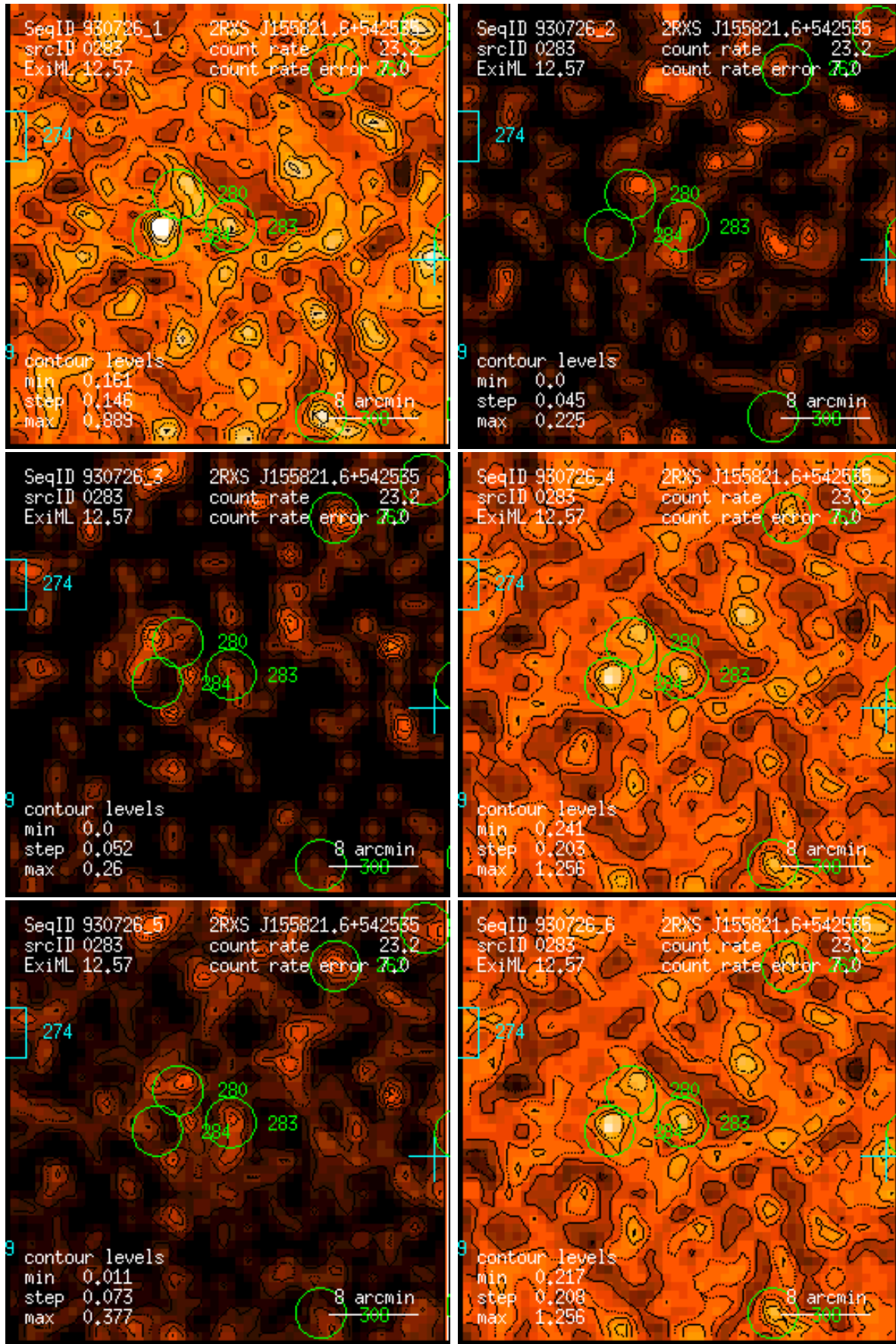
Figure 283: RASS 930726: detection 0283: band rate images, Gaussian filter: (1) PSPC channels 11 – 41, (2) 52 – 90, (3) 91 – 201, (4) 11 – 235, (5) 52 – 201, (6) 11 – 201. Broad band rates in counts/ks. Band rate contour levels in counts/ks/arcmin 2 .
