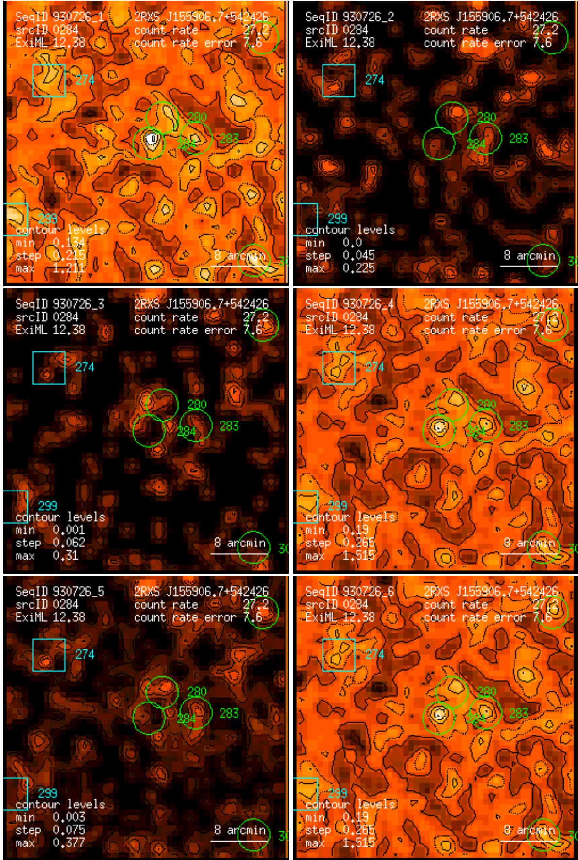
Figure 284: RASS 930726: detection 0284: band rate images, Gaussian filter: (1) PSPC channels 11 – 41, (2) 52 – 90, (3) 91 – 201, (4) 11 – 235, (5) 52 – 201, (6) 11 – 201. Broad band rates in counts/ks. Band rate contour levels in counts/ks/arcmin 2 .
