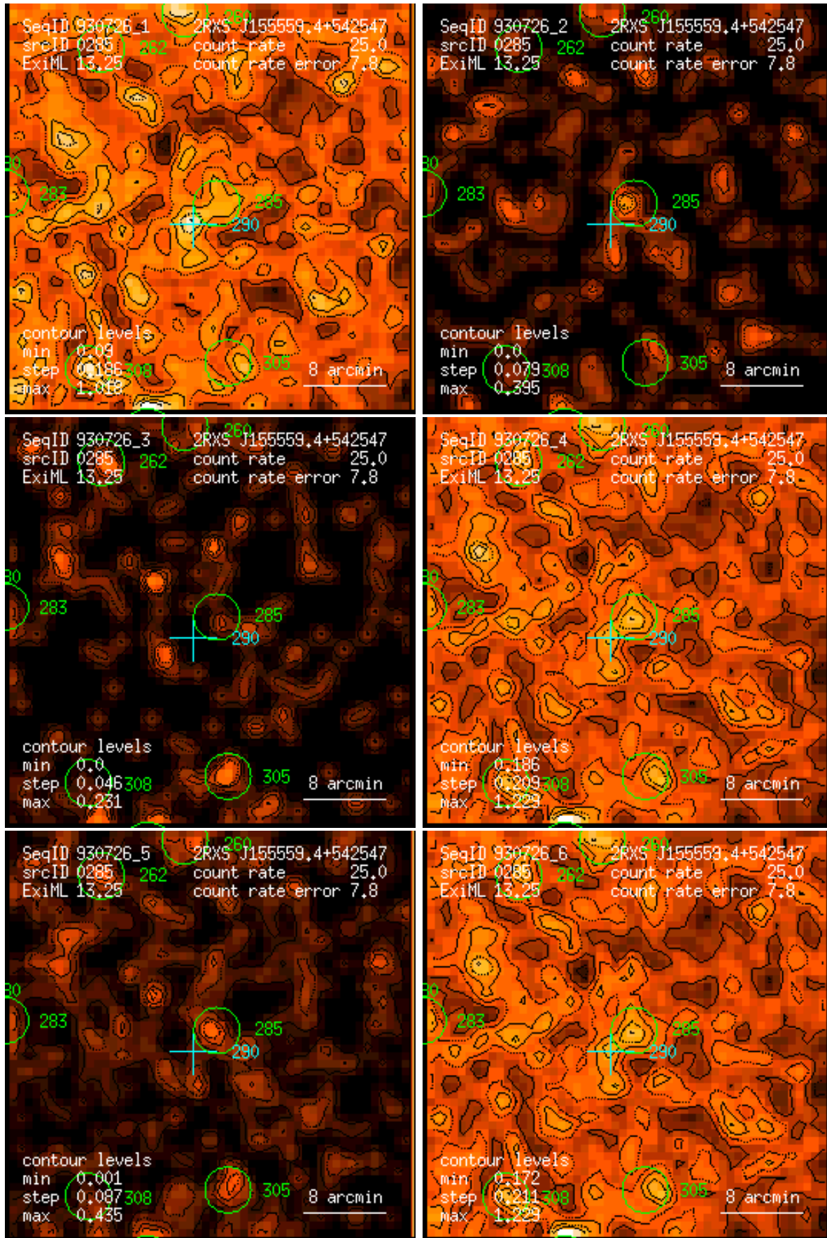
Figure 285: RASS 930726: detection 0285: band rate images, Gaussian filter: (1) PSPC channels 11 – 41, (2) 52 – 90, (3) 91 – 201, (4) 11 – 235, (5) 52 – 201, (6) 11 – 201. Broad band rates in counts/ks. Band rate contour levels in counts/ks/arcmin 2 .
