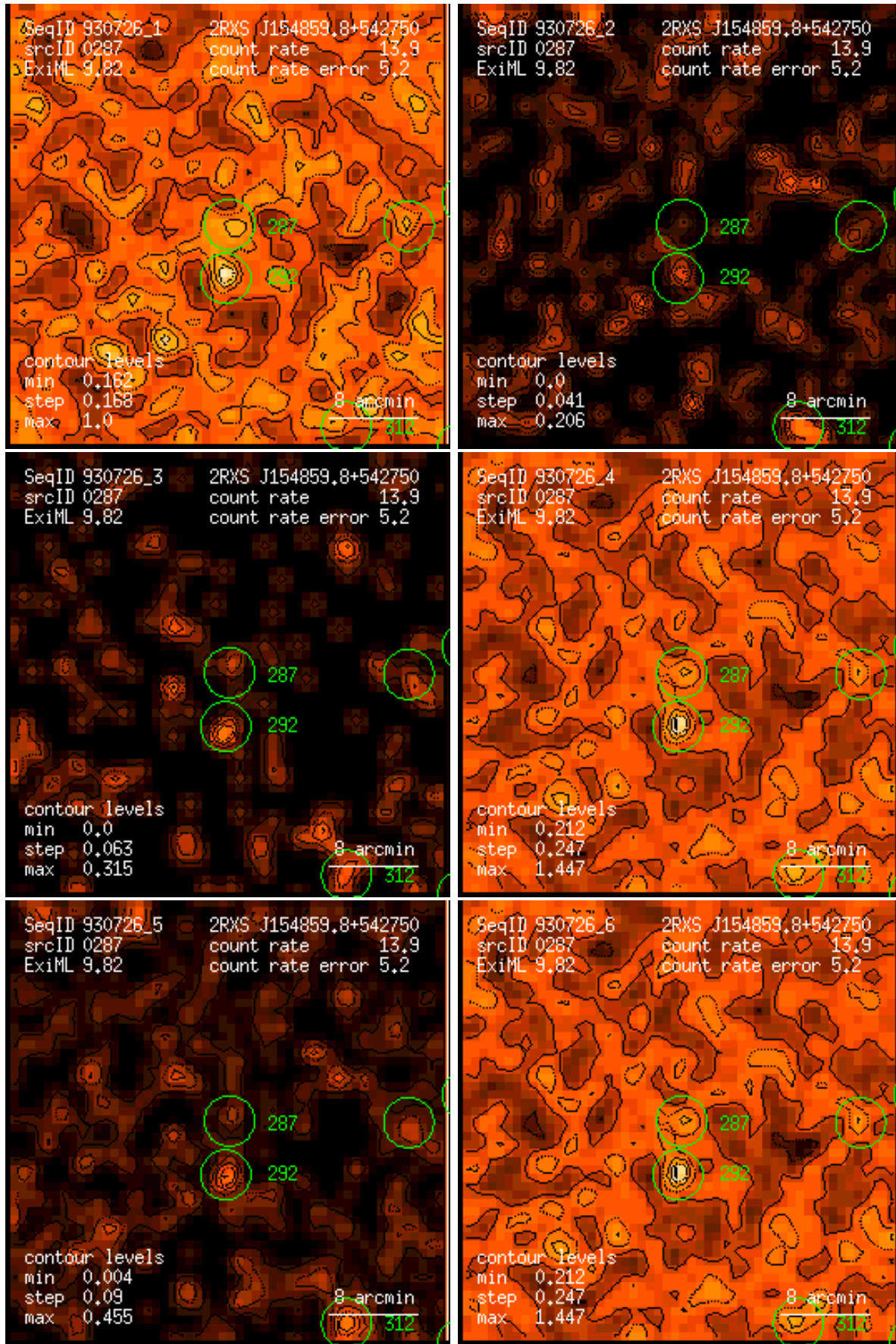
Figure 287: RASS 930726: detection 0287: band rate images, Gaussian filter: (1) PSPC channels 11 – 41, (2) 52 – 90, (3) 91 – 201, (4) 11 – 235, (5) 52 – 201, (6) 11 – 201. Broad band rates in counts/ks. Band rate contour levels in counts/ks/arcmin 2 .
