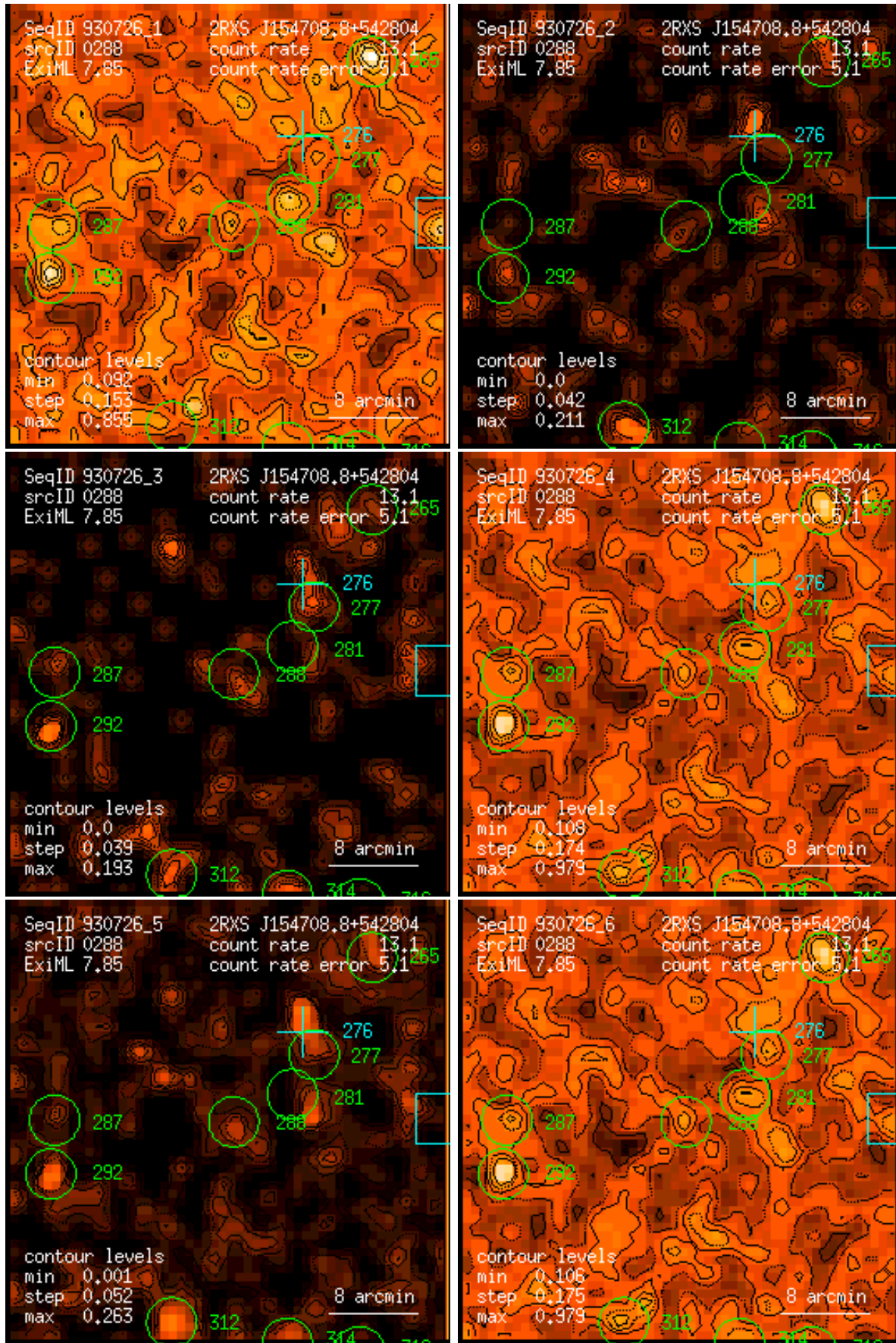
Figure 288: RASS 930726: detection 0288: band rate images, Gaussian filter: (1) PSPC channels 11 – 41, (2) 52 – 90, (3) 91 – 201, (4) 11 – 235, (5) 52 – 201, (6) 11 – 201. Broad band rates in counts/ks. Band rate contour levels in counts/ks/arcmin 2 .
